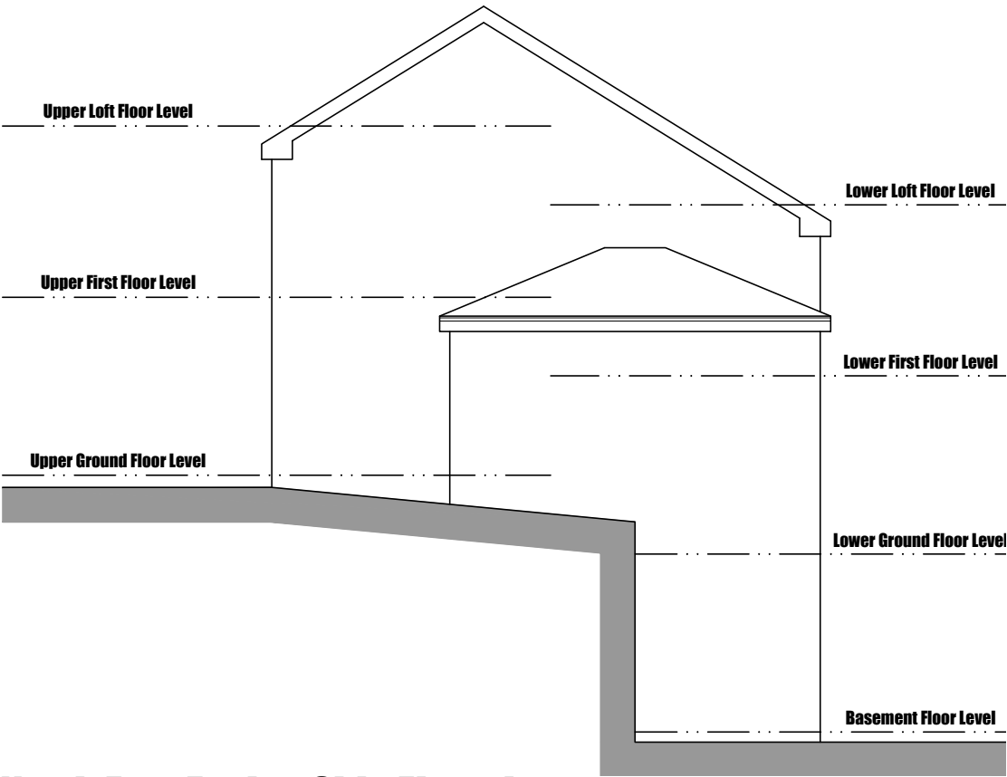
North East Facing Side Elevation
