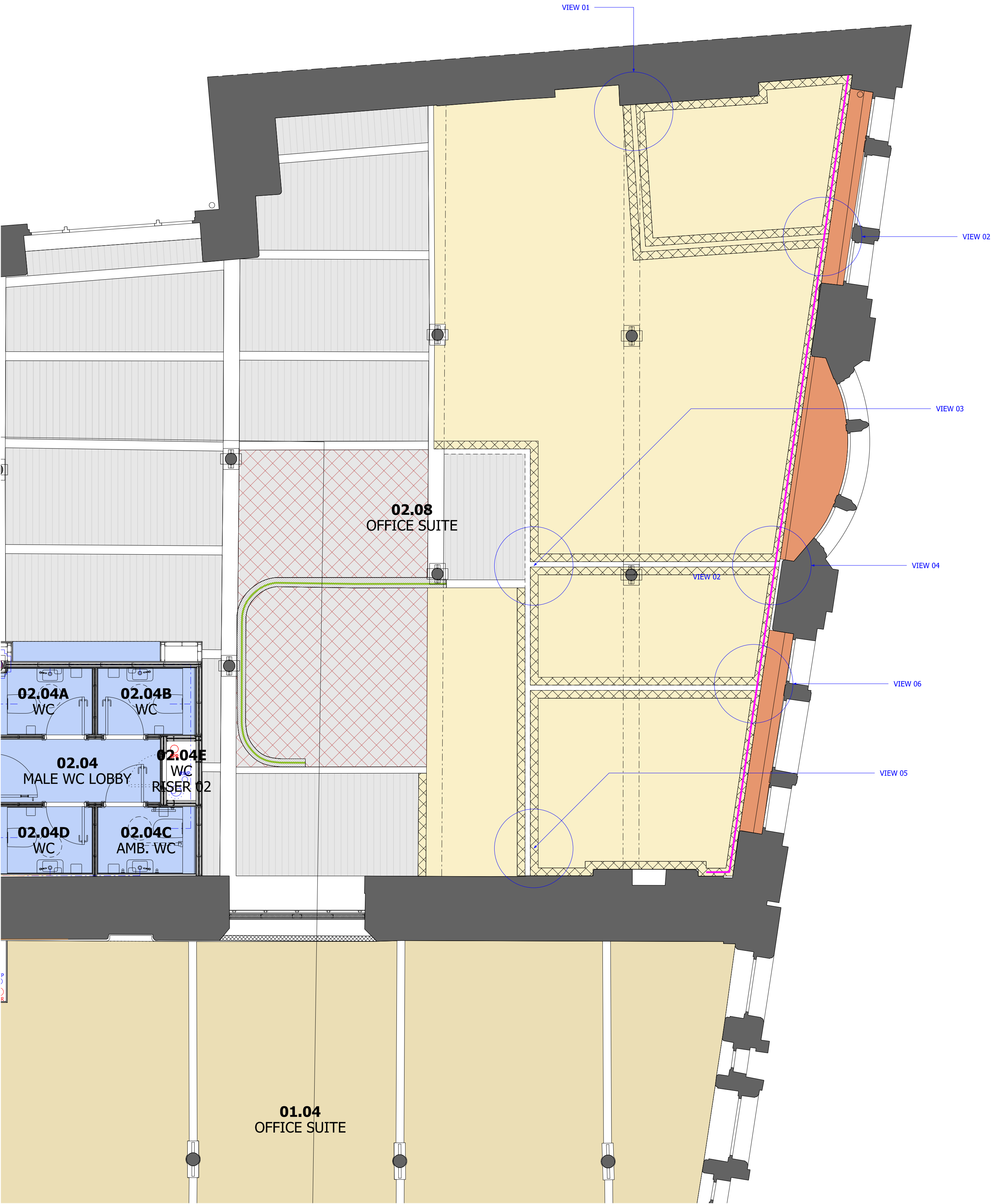
Part RCP layout: Level 02
