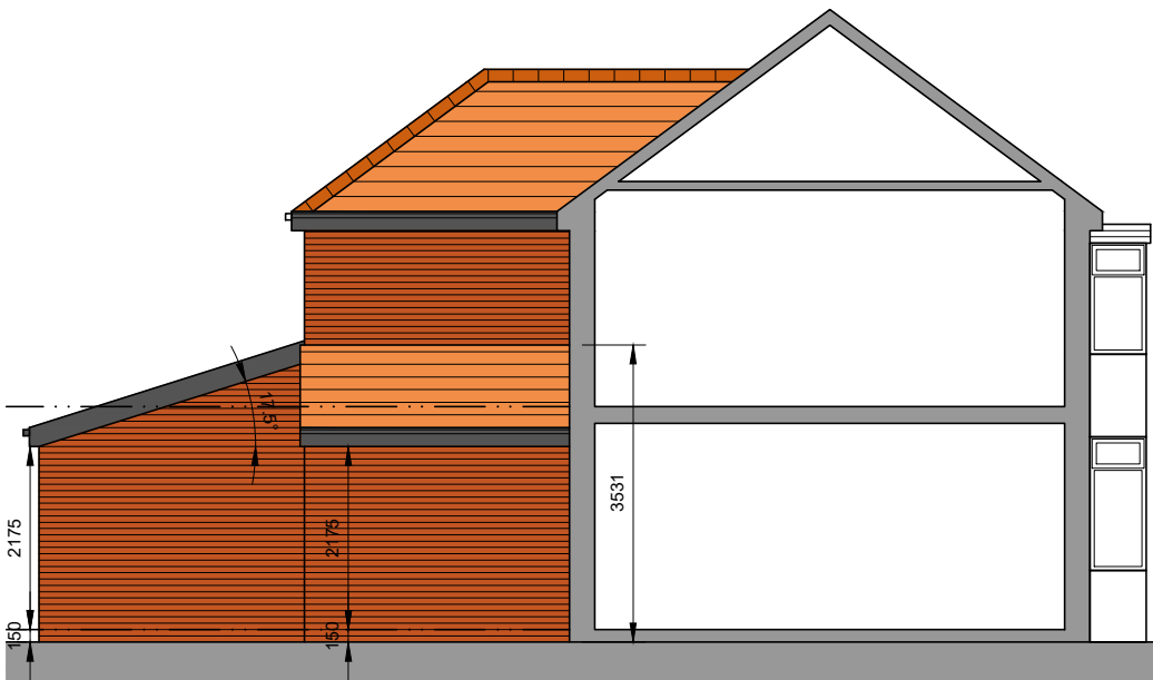
East Facing Side Elevational Section
