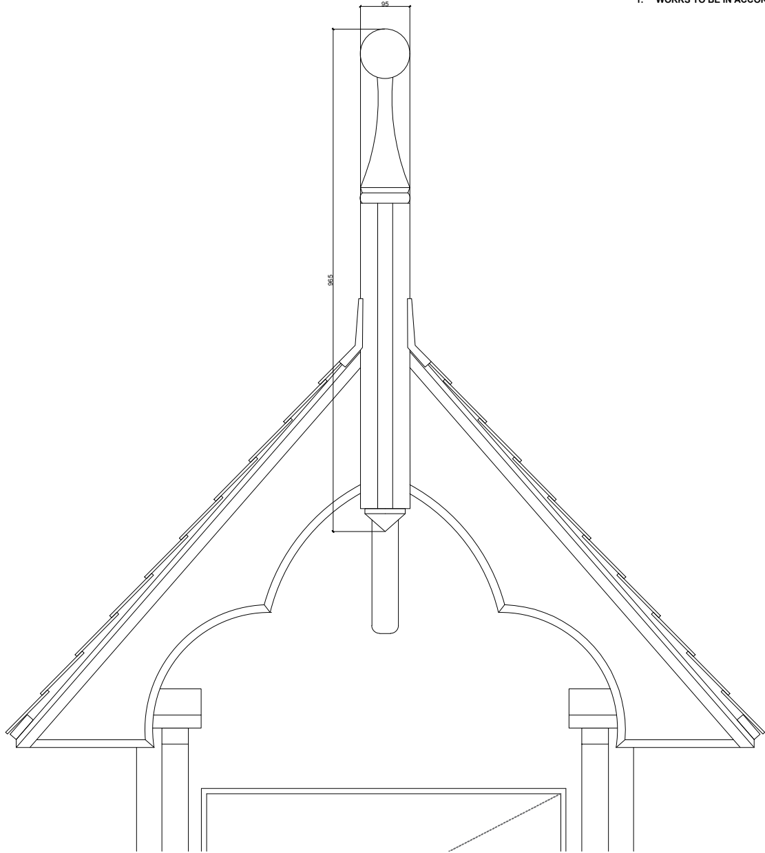
1 Roof finial 1:10
