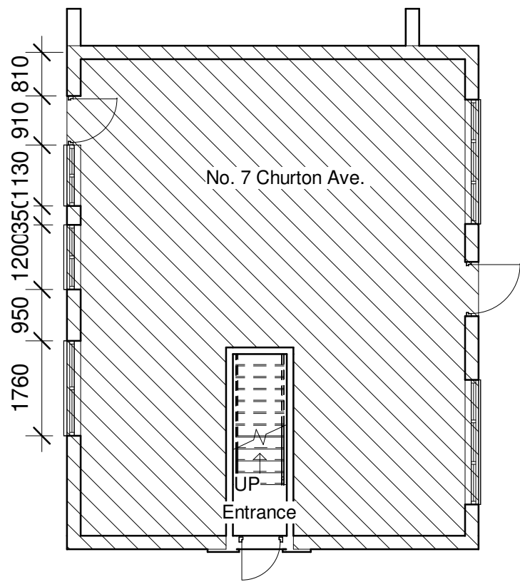
1 Ground Floor - Existing 1 : 100
