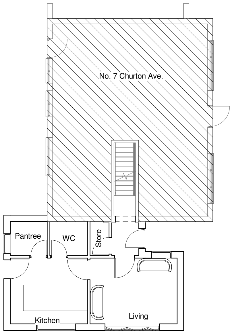
2 Ground Floor - Proposed 1 : 100
