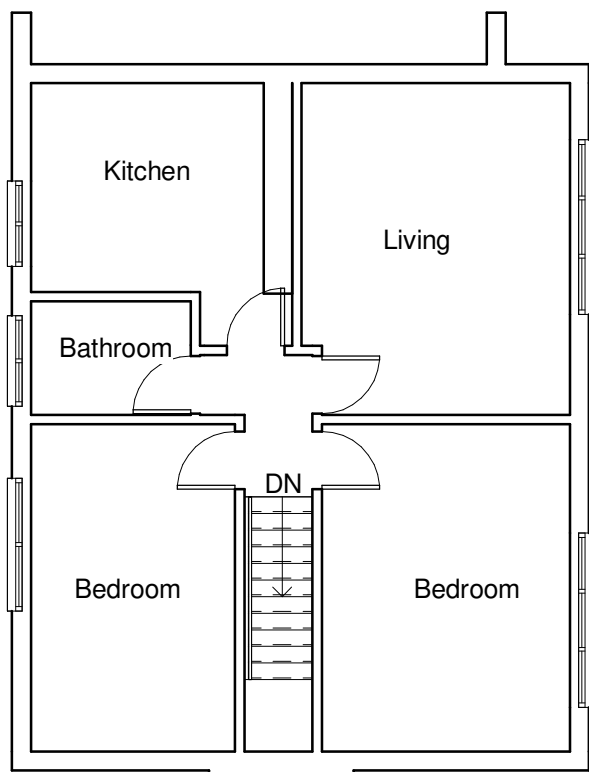
3 First Floor- Existing 1 : 100
