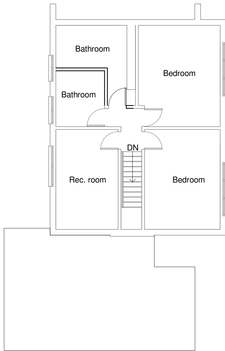
4 First Floor- Proposed 1 : 100
