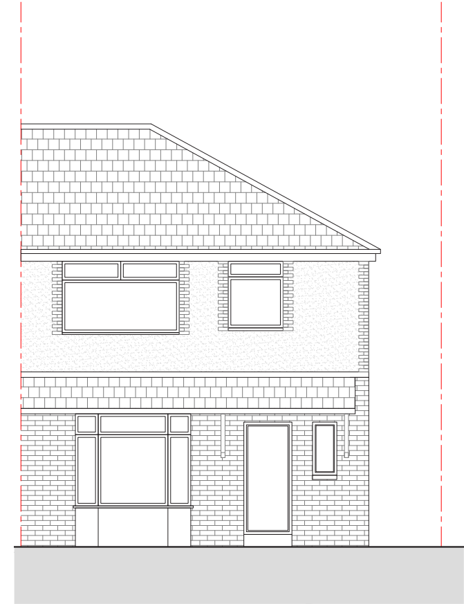
EXISTING FRONT ELEVATION 1:100 @ A3
