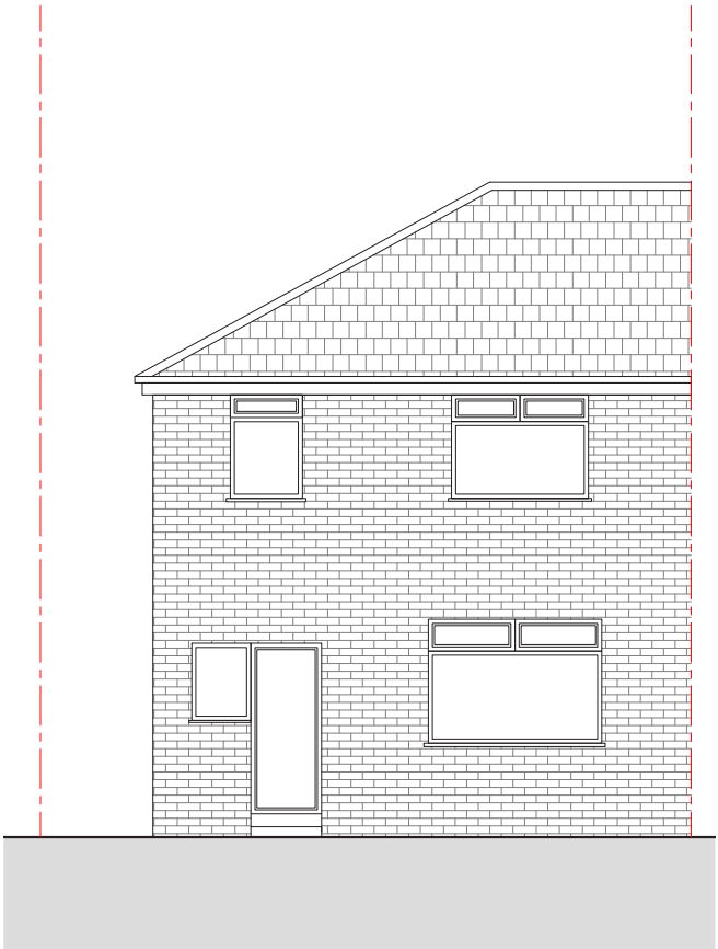
EXISTING REAR ELEVATION 1:100 @ A3
