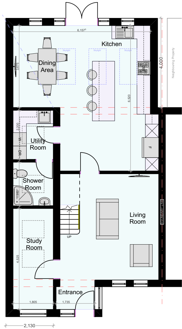
PROPOSED GA GROUND FLOOR PLAN
