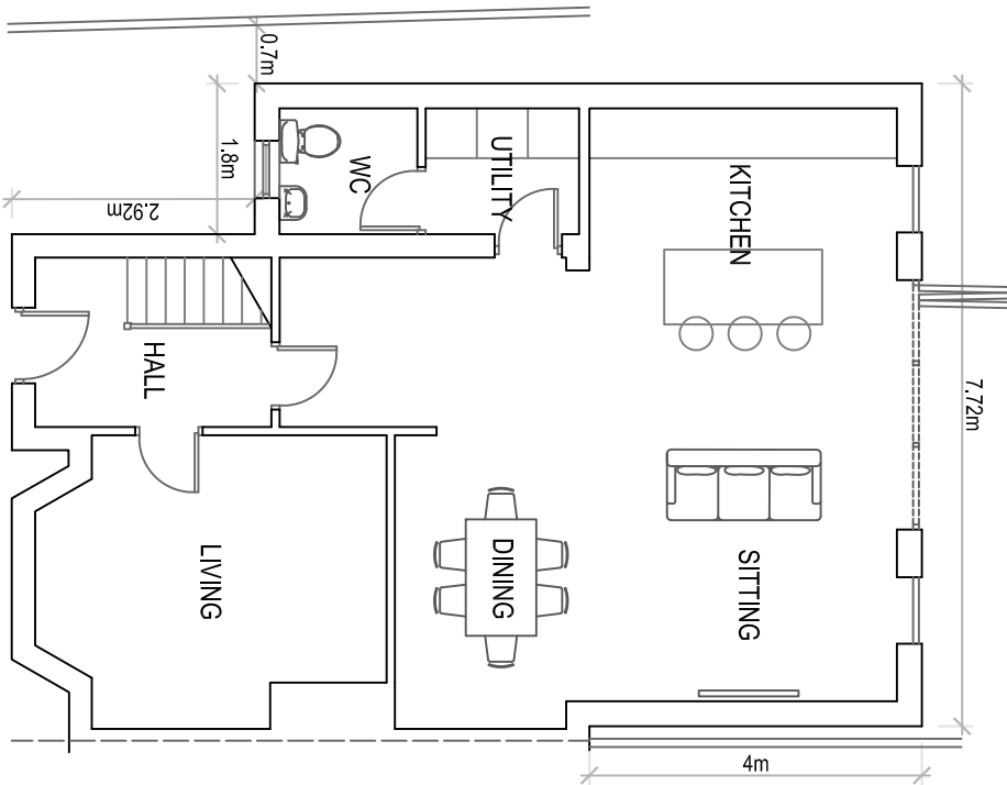
PROPOSED GF PLAN 1:100
