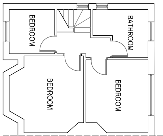
PROPOSED FF PLAN 1:100
