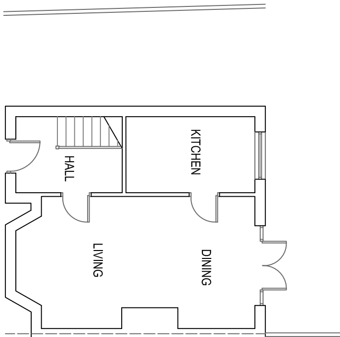
EXISTING GF PLAN 1:100
