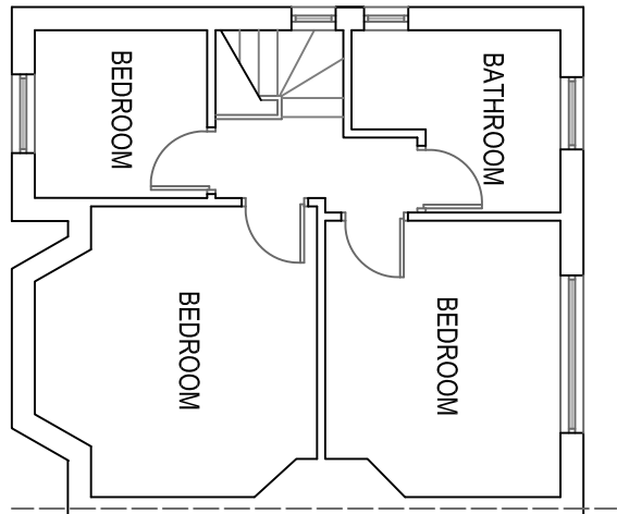
EXISTING FF PLAN 1:100
