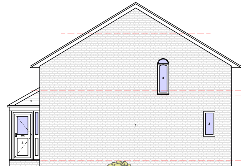
EXISTING GA SIDE ELEVATION 1 @1:100
