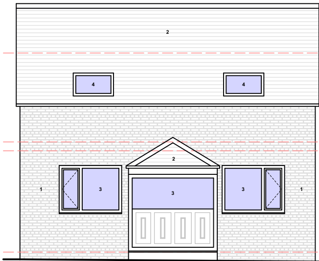
EXISTING GA FRONT ELEVATION @1:100
