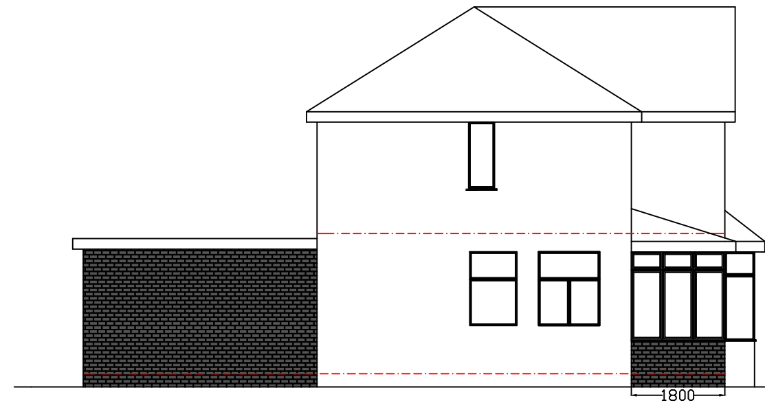
Side Elevation
