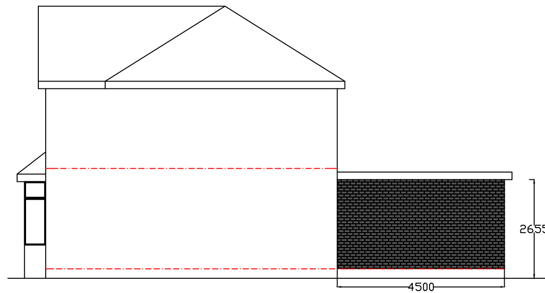
Side Elevation From No 7
