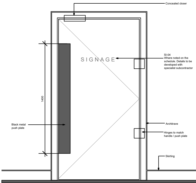
Type C3 : Front Elevation, Single Arrangement
