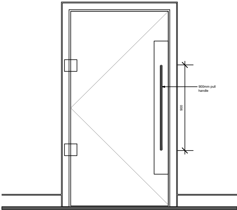
Type C3 : Rear Elevation, Single Arrangement
