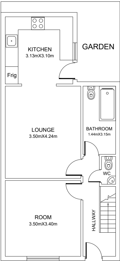
EXISTING GROUND FLOOR
