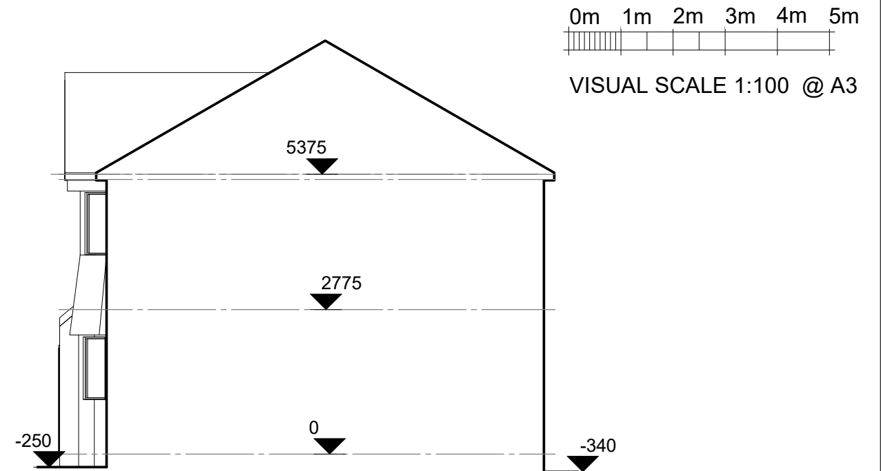
02-E-Elevation 1 : 100
