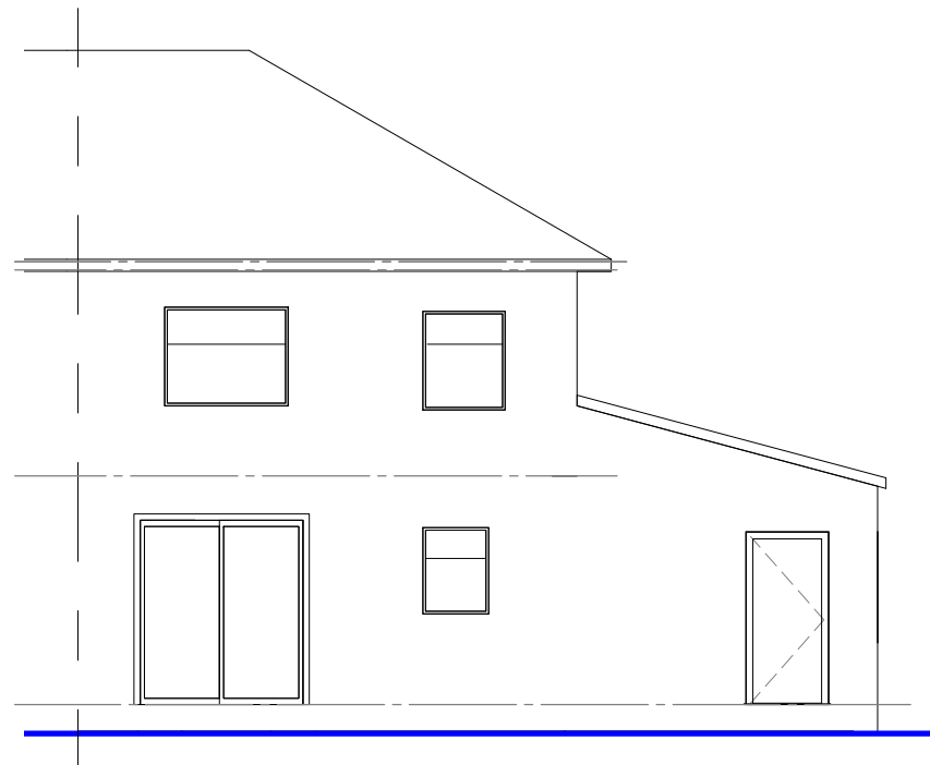
03-E-Elevation 1 : 100
