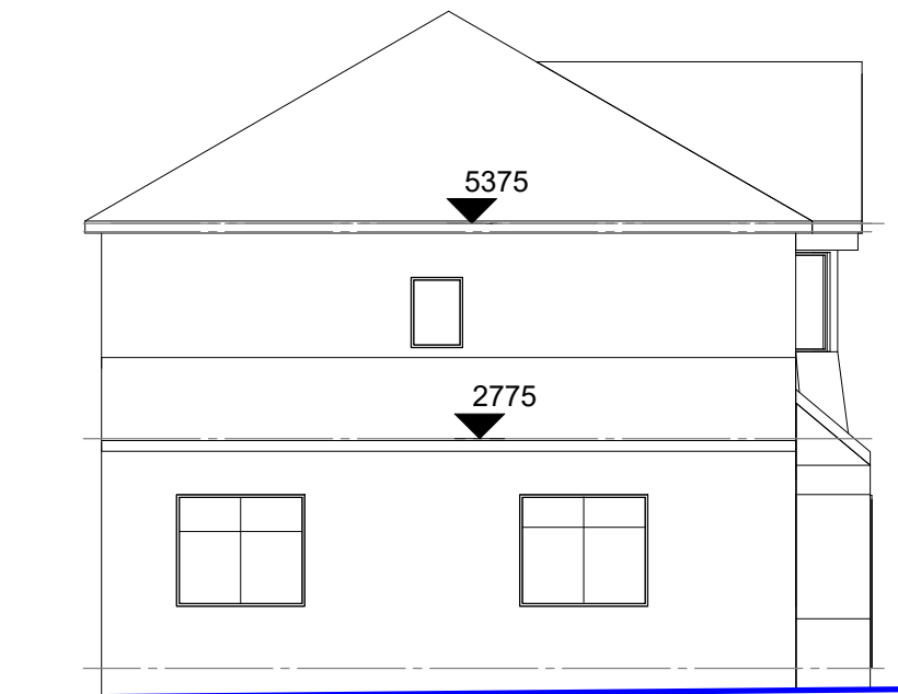
04-E-Elevation 1 : 100
