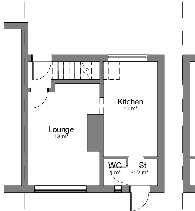
00-E-Ground Floor 1 : 100
