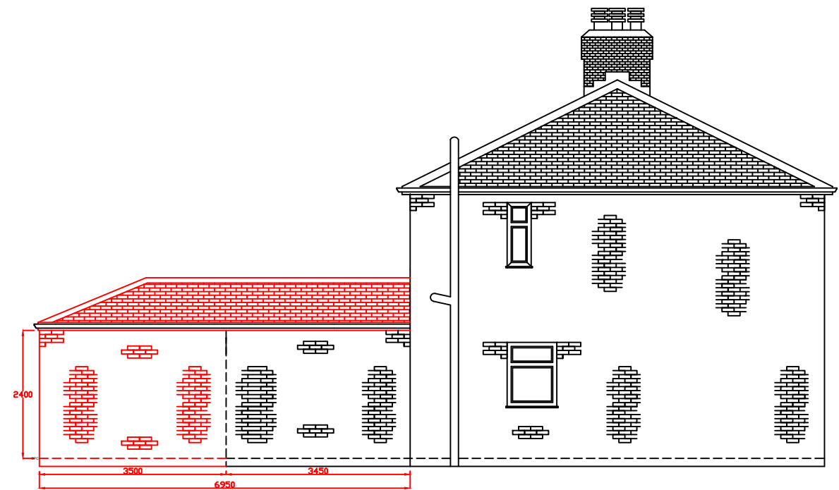
PROPOSED SIDE ELEVATION (B) - Ref : 007
