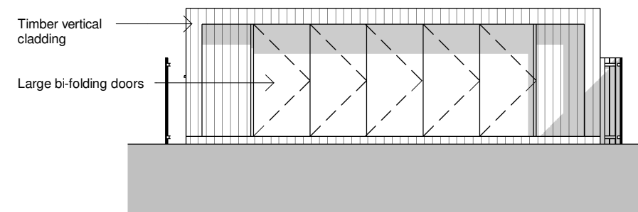
5 Outbuilding - South Elevation 1 : 100
