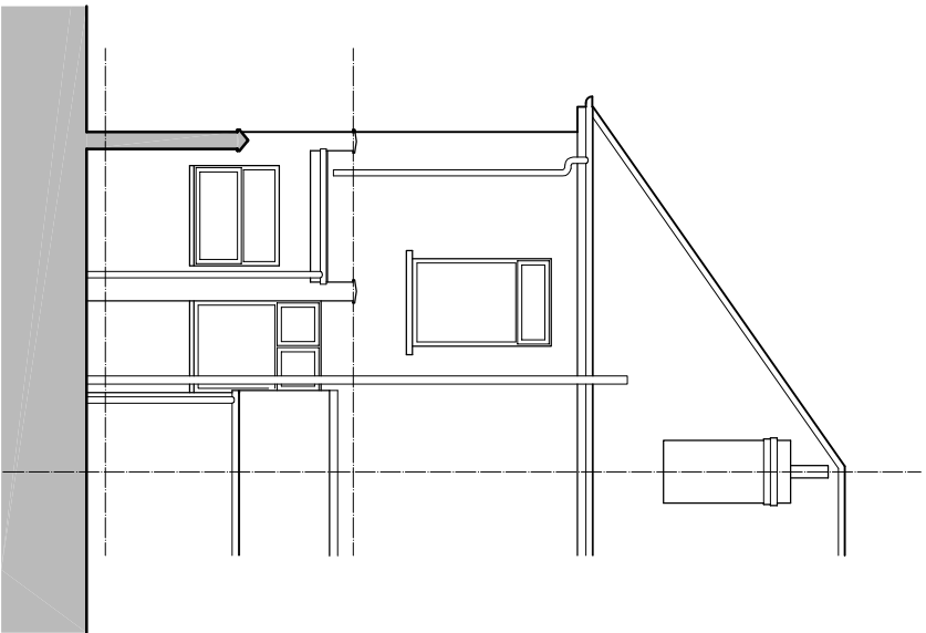
REAR ELEVATION 1:100
