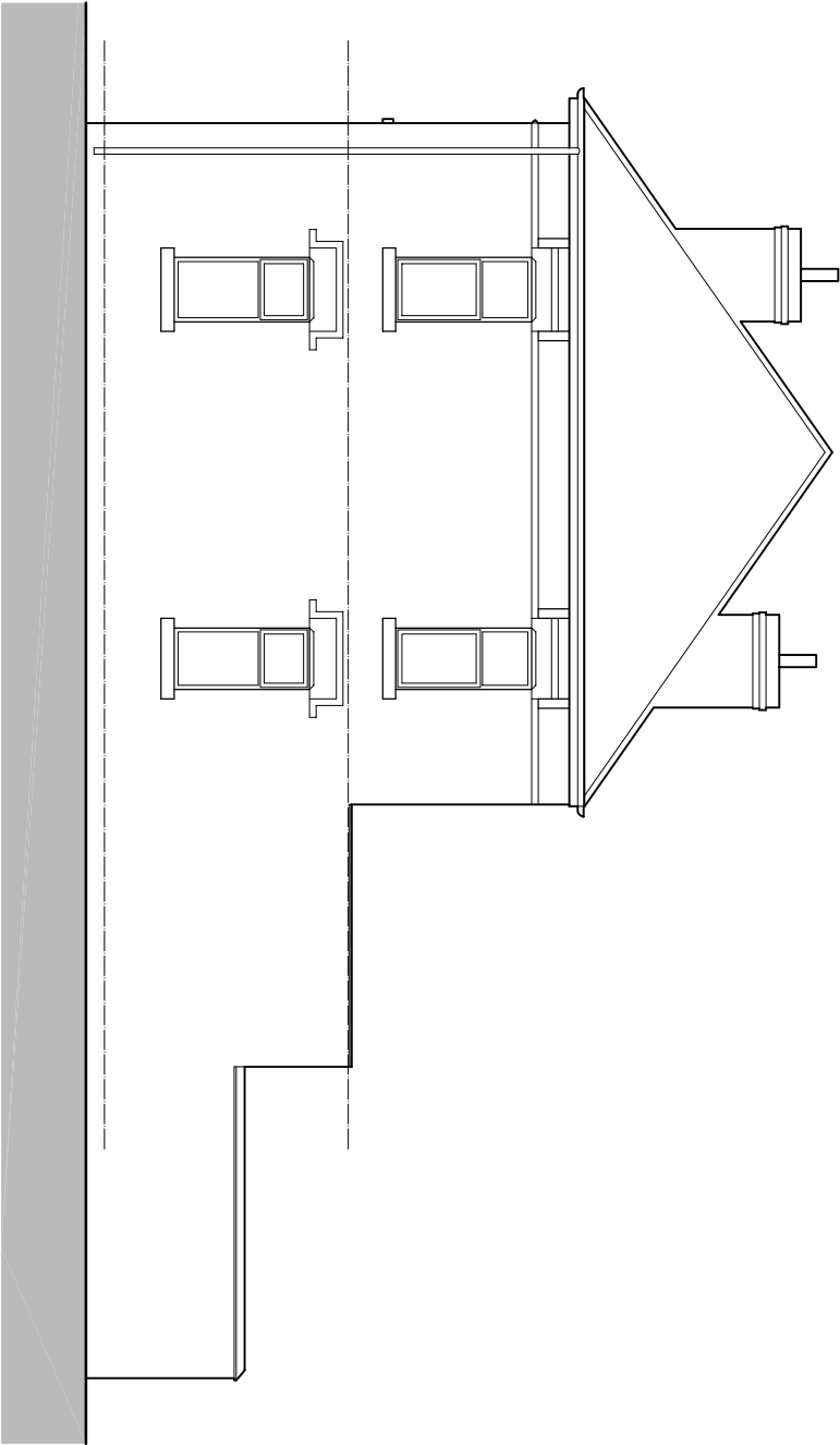
SIDE / EDWARD AVENUE ELEVATION 1:100
