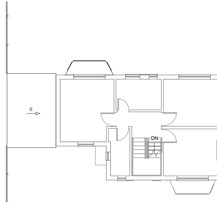
2 First Floor Plan 1 : 150
