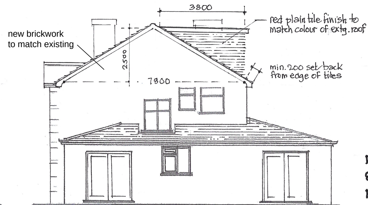
SIDE ELEVATION
