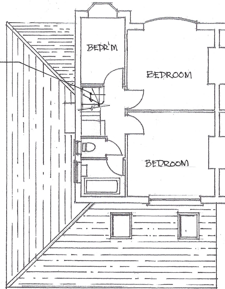
FIRST FLOOR
