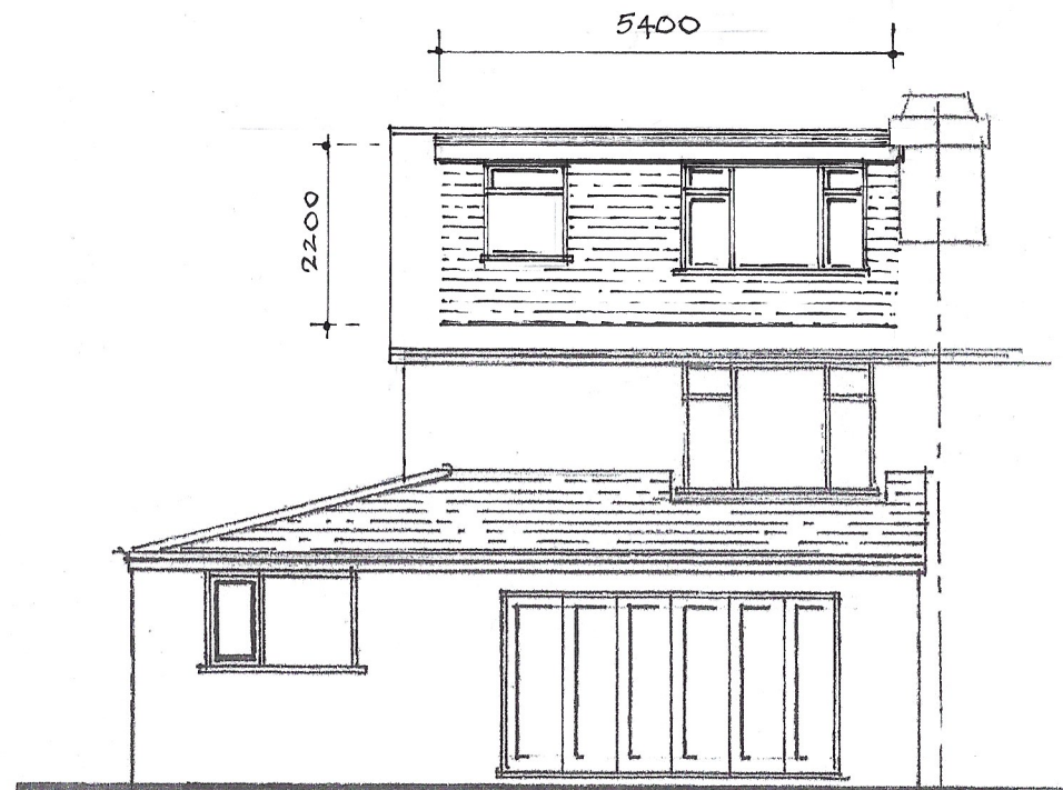
REAR ELEVATION
