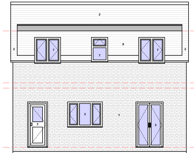
PROPOSED GA REAR ELEVATION @1:100
