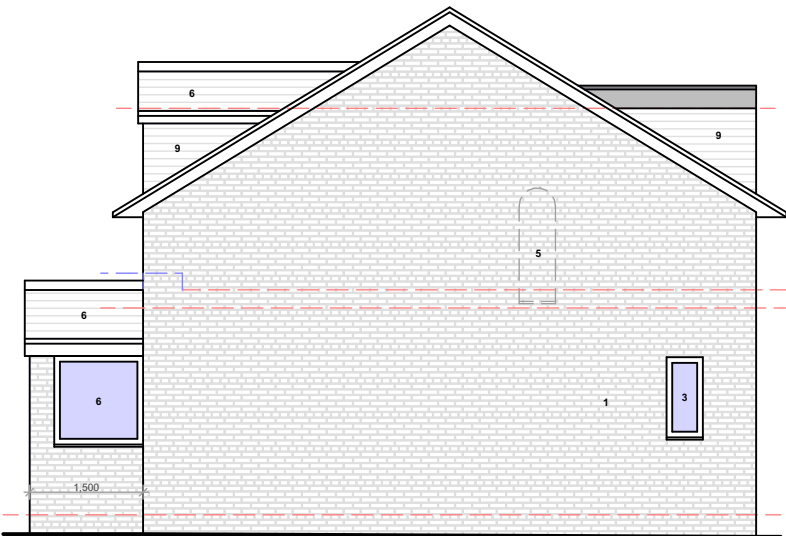
PROPOSED GA SIDE ELEVATION 1 @1:100
