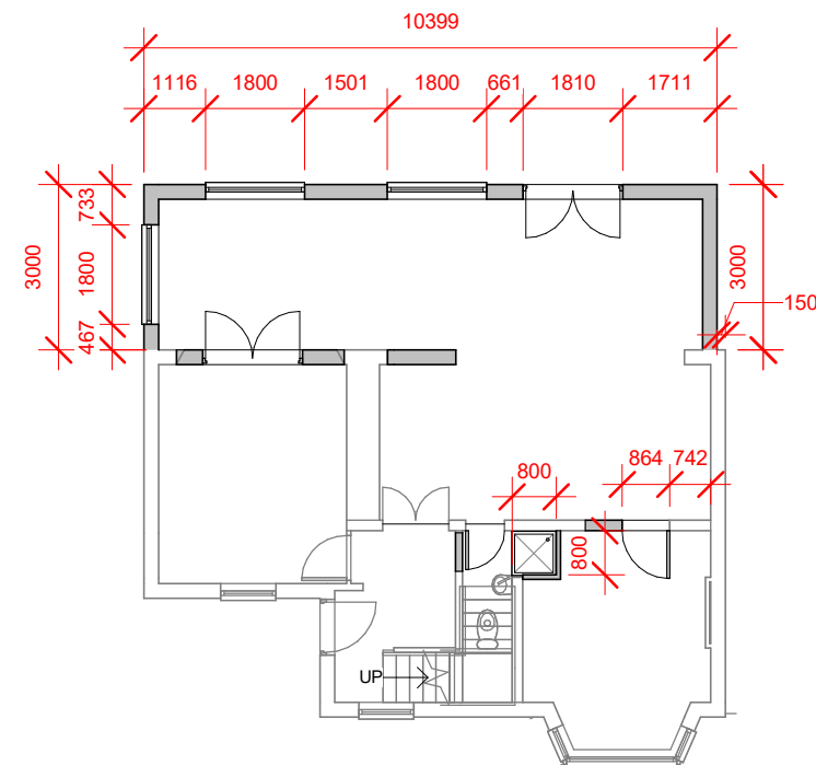
1 Ground Floor Plan 1 : 150
