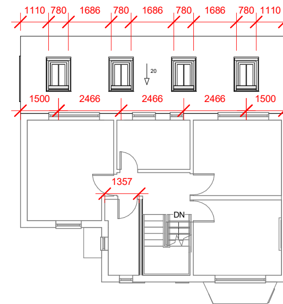
2 First Floor Plan 1 : 150
