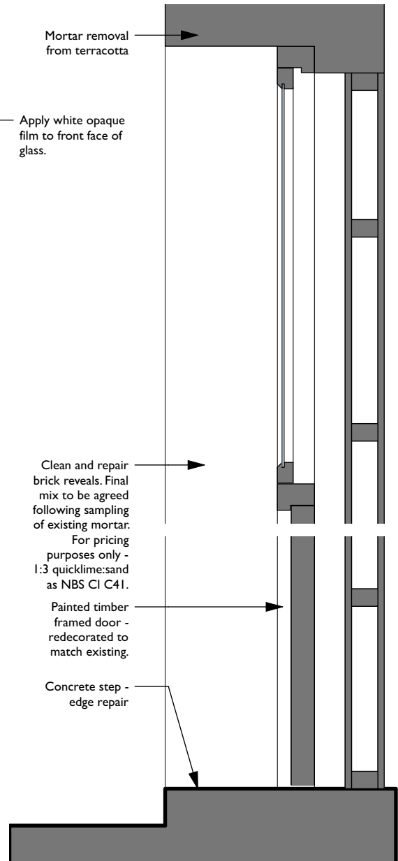
5 Proposed Cill Detail Scale: 1:10
