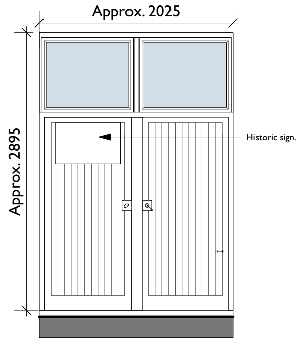
1 Existing Door Elevation Scale: 1:40 Approx. 2025
