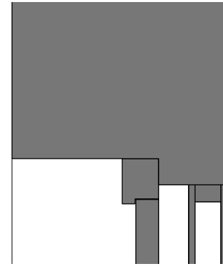
3 Existing Jamb Detail Scale: 1:10
