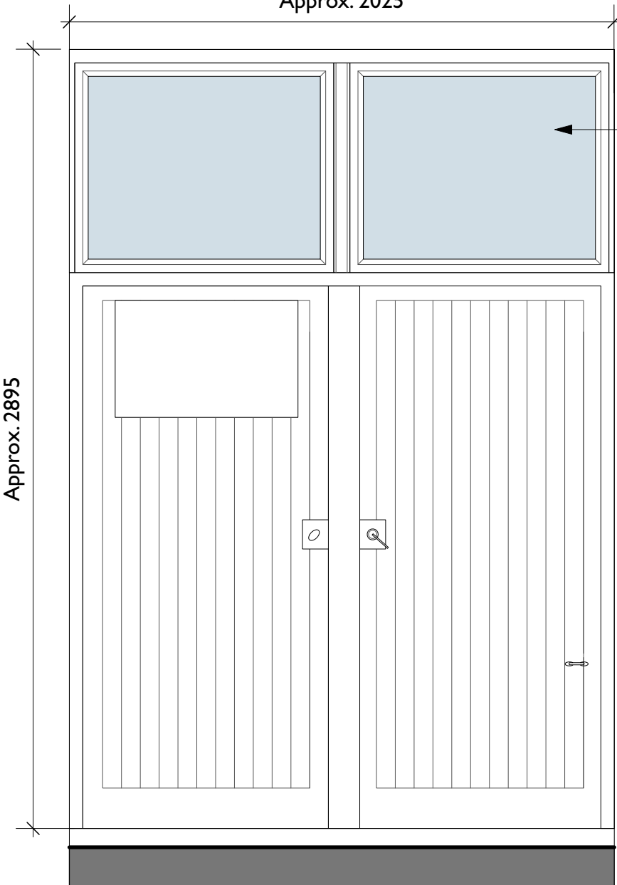
4 Proposed Door Elevation Scale: 1:20
