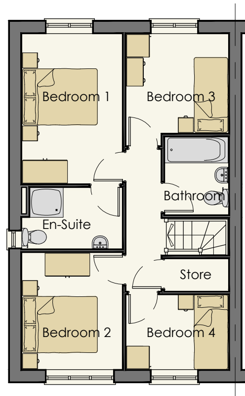
First Floor Plan 4B5P House Type 100sq.m
