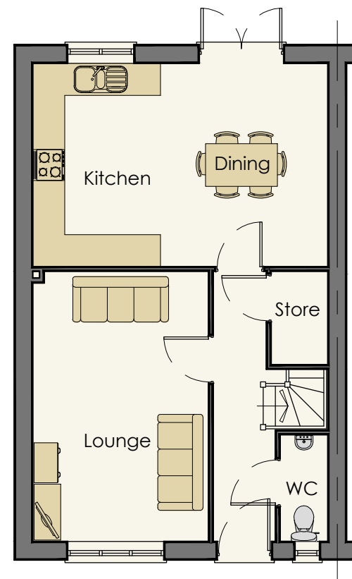
Ground Floor Plan 4B5P House Type 100sq.m
