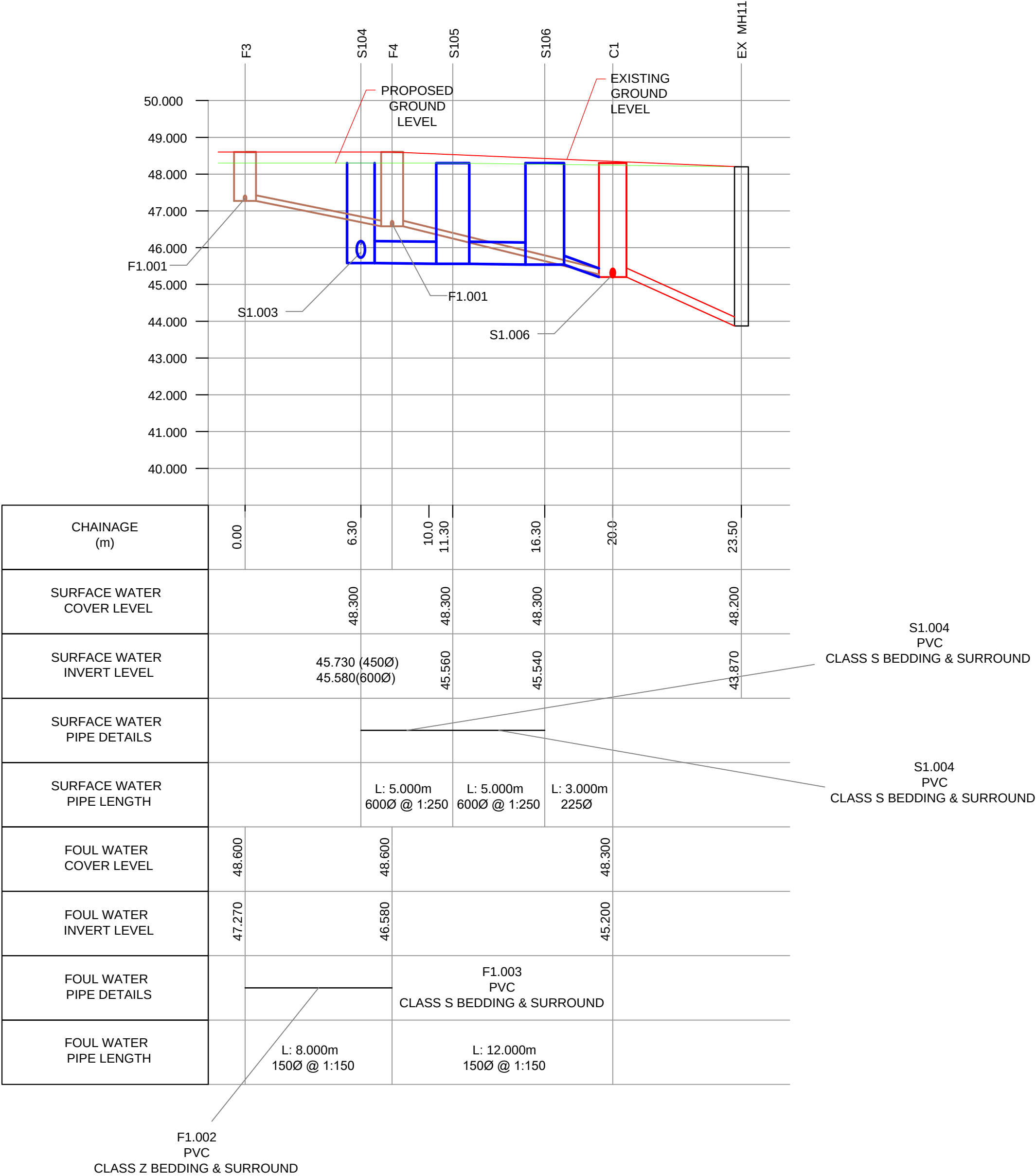
LONG SECTION MH F3 - EXISTING MH11
