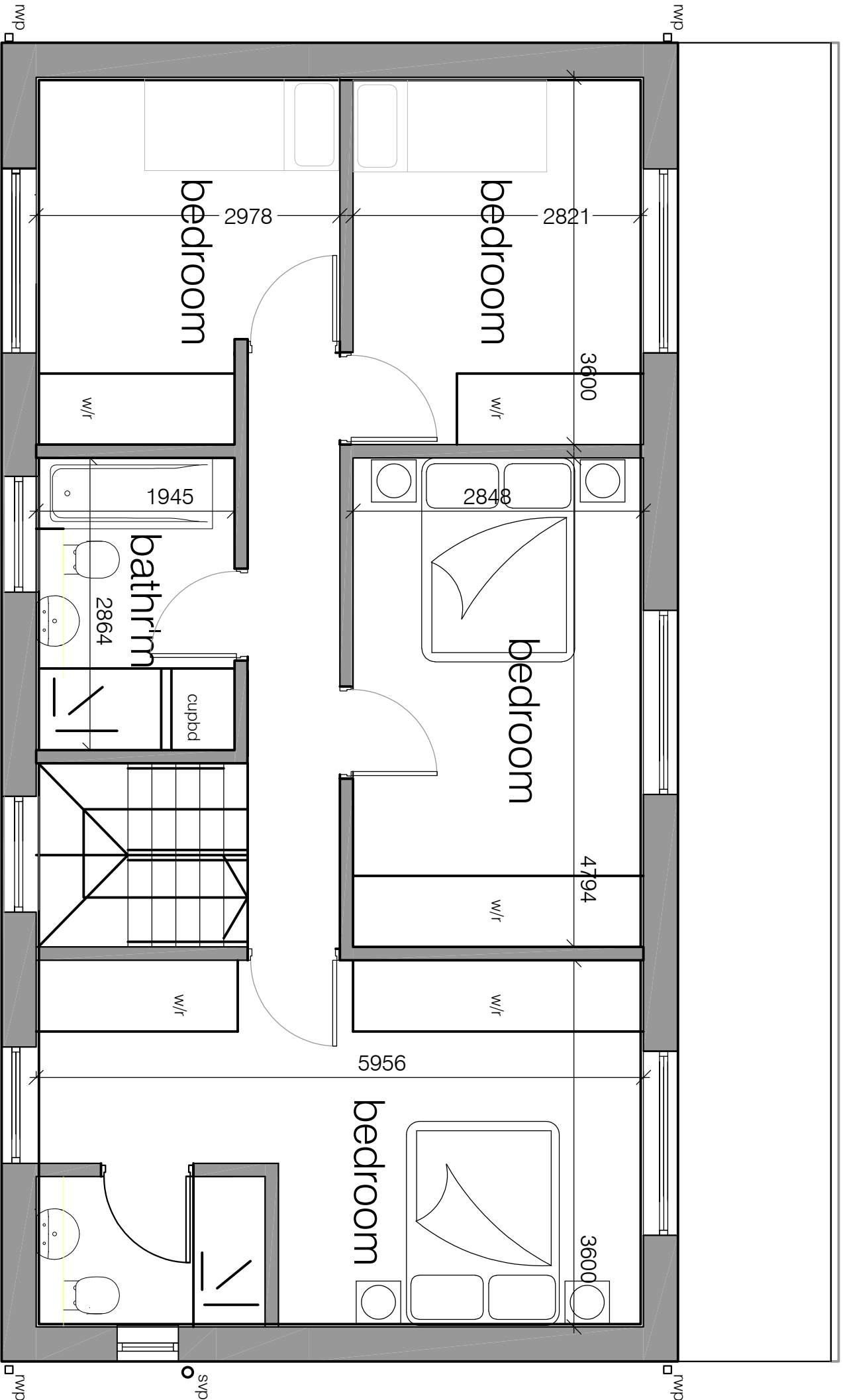
First Floor 71.9m2 G.I.A (773 sq ft)
