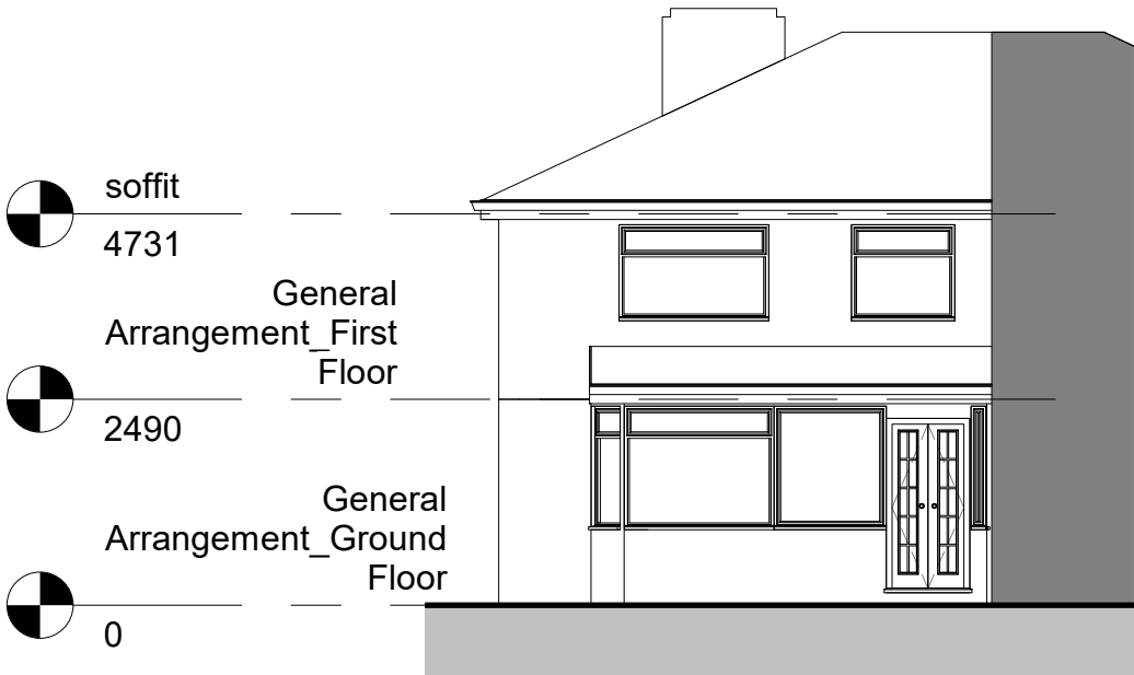
Existing Elevation South 1 : 100
