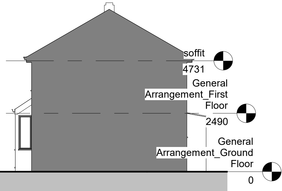
Existing Elevation East 1 : 100
