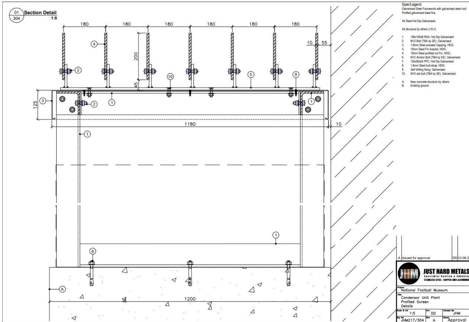
Figure 5- Fabrication drawing cross section of structure
