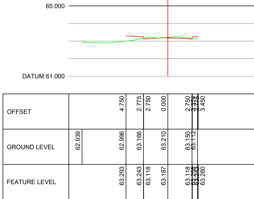
ALIGNMENT ROAD1 CHAINAGE 80.000
