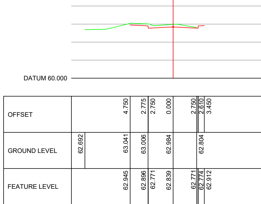
ALIGNMENT ROAD1 CHAINAGE 120.000
