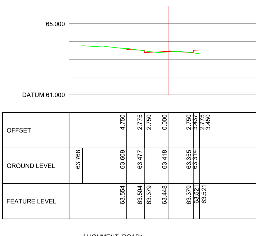
ALIGNMENT ROAD1 CHAINAGE 50.000
