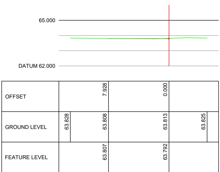
ALIGNMENT ROAD1 CHAINAGE 0.000
