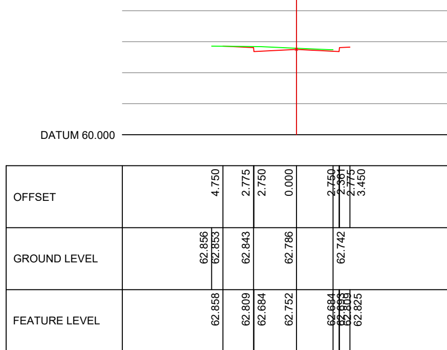
ALIGNMENT ROAD1 CHAINAGE 130.000
