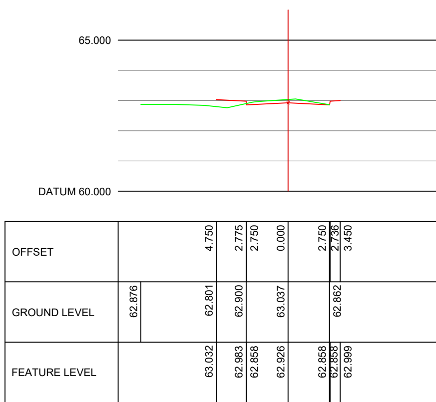
ALIGNMENT ROAD1 CHAINAGE 110.000
