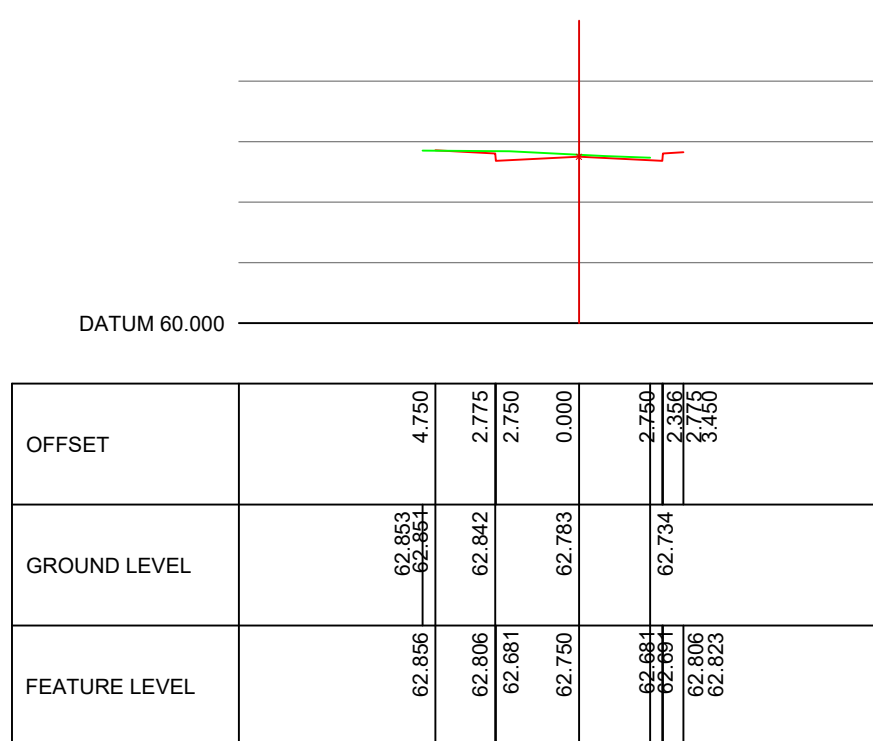
ALIGNMENT ROAD1 CHAINAGE 130.268
