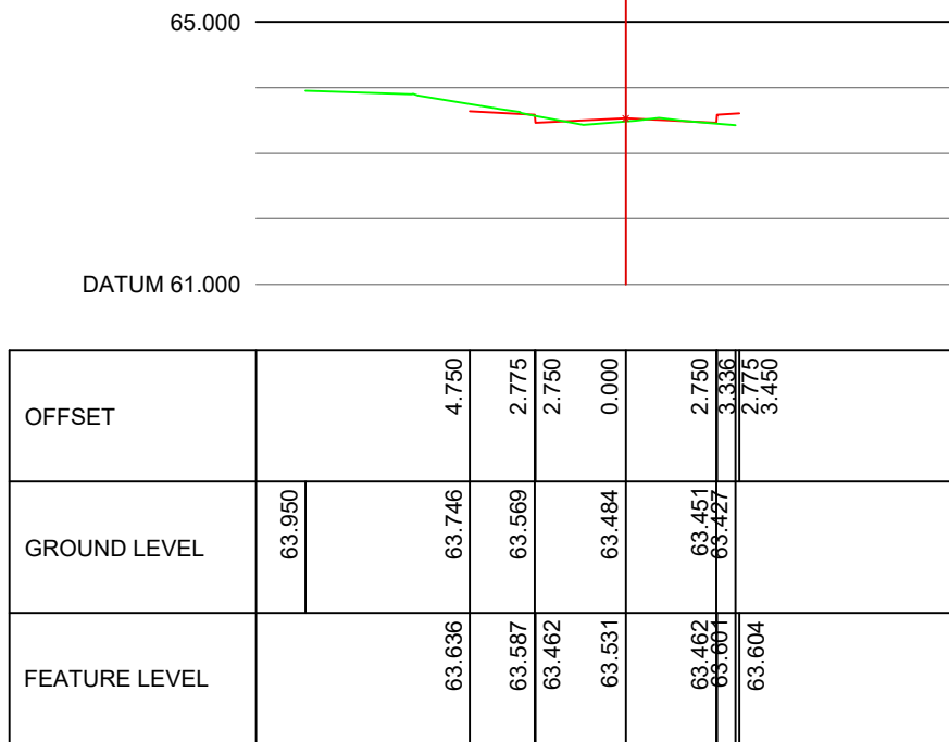
ALIGNMENT ROAD1 CHAINAGE 40.000
