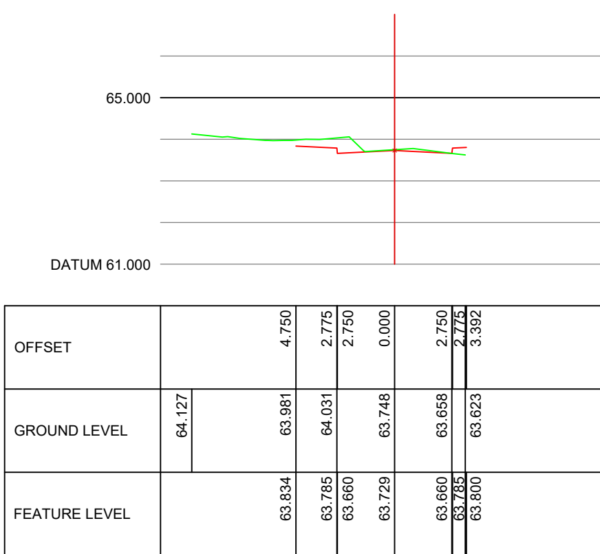
ALIGNMENT ROAD1 CHAINAGE 10.000
