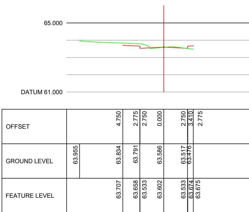
ALIGNMENT ROAD1 CHAINAGE 30.000
