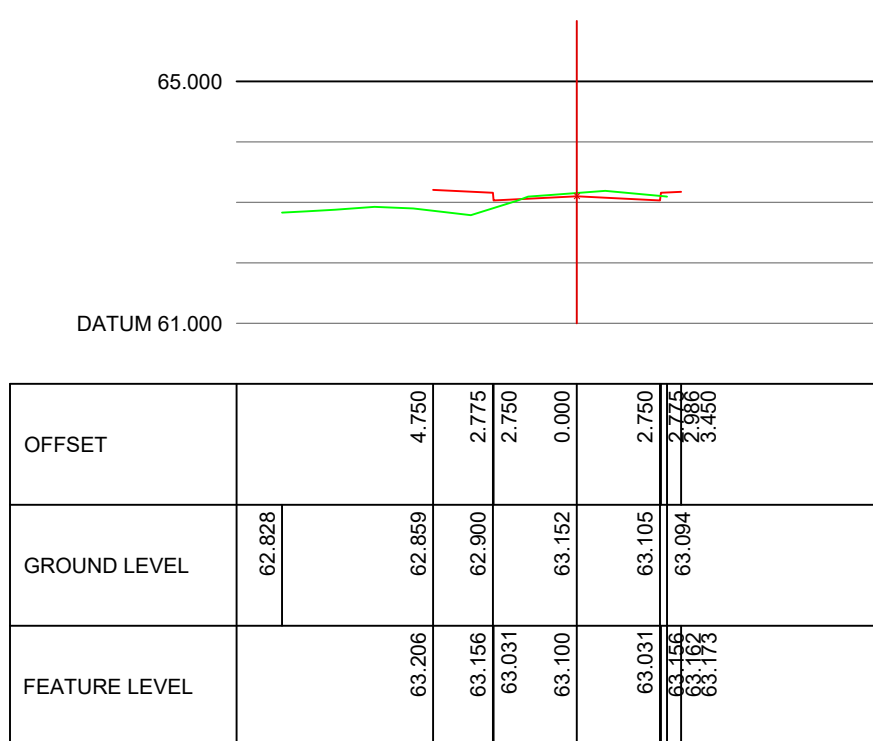
ALIGNMENT ROAD1 CHAINAGE 90.000
