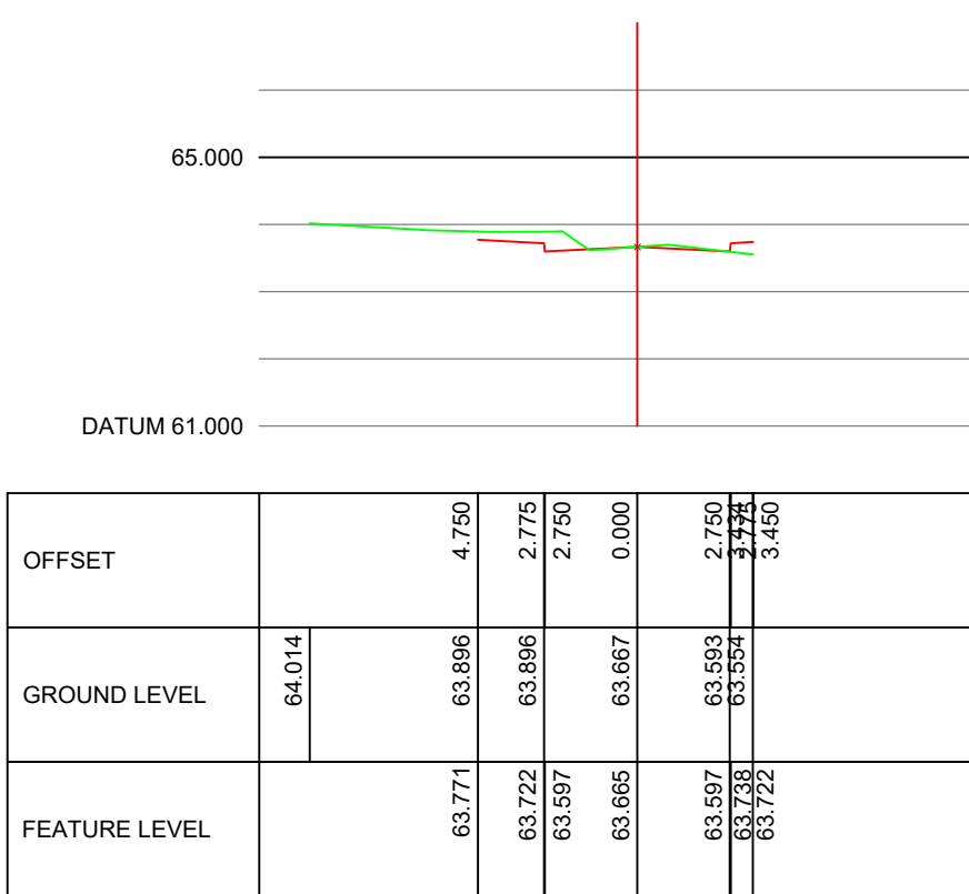
ALIGNMENT ROAD1 CHAINAGE 20.000
