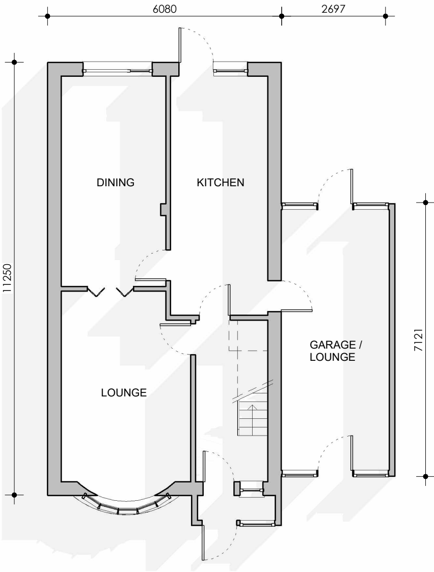
GROUND FLOOR PLAN @1:50
