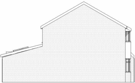
LEFT ELEVATION @1:200
