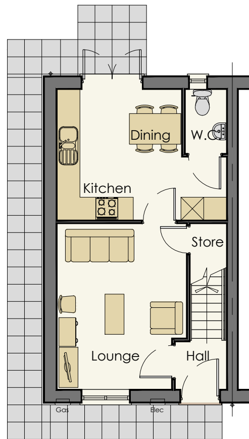
Ground Floor Plan 2B3P House Type 70sq.m
