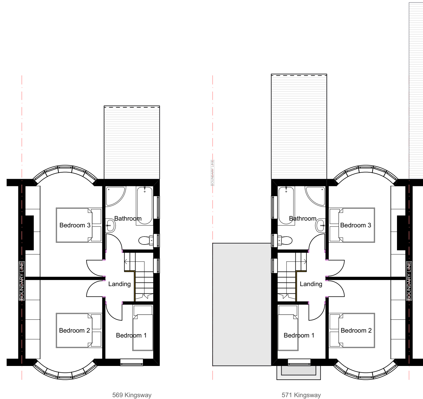
EXISTING GA FIRST FLOOR PLANS
