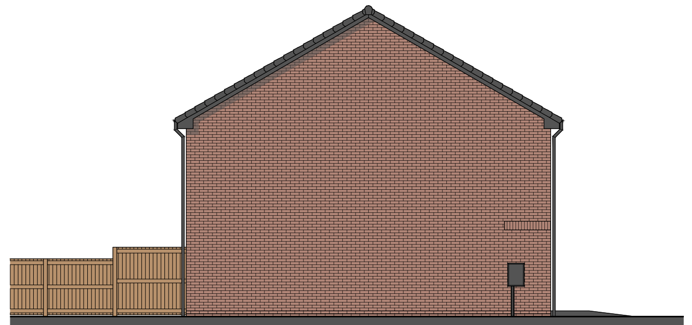
Side Elevation 3B4P House Type 87sq.m (Adjoining property handed)
