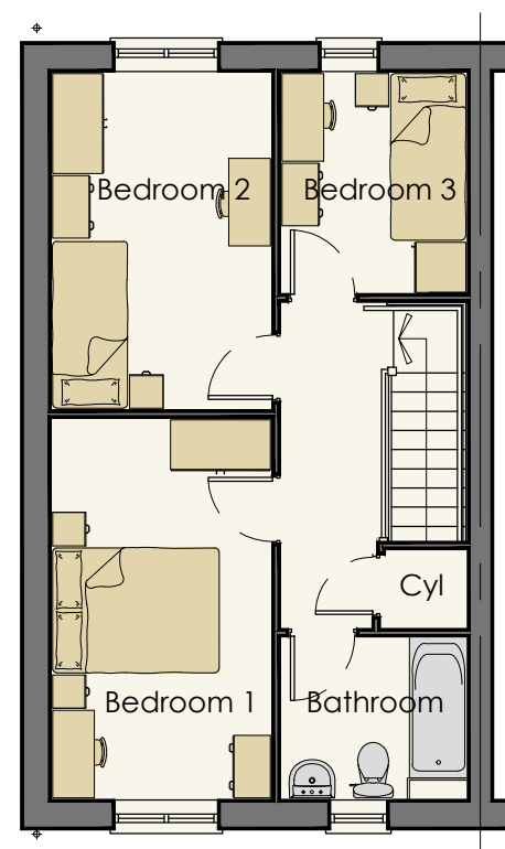
First Floor Plan 3B4P House Type 87sq.m
