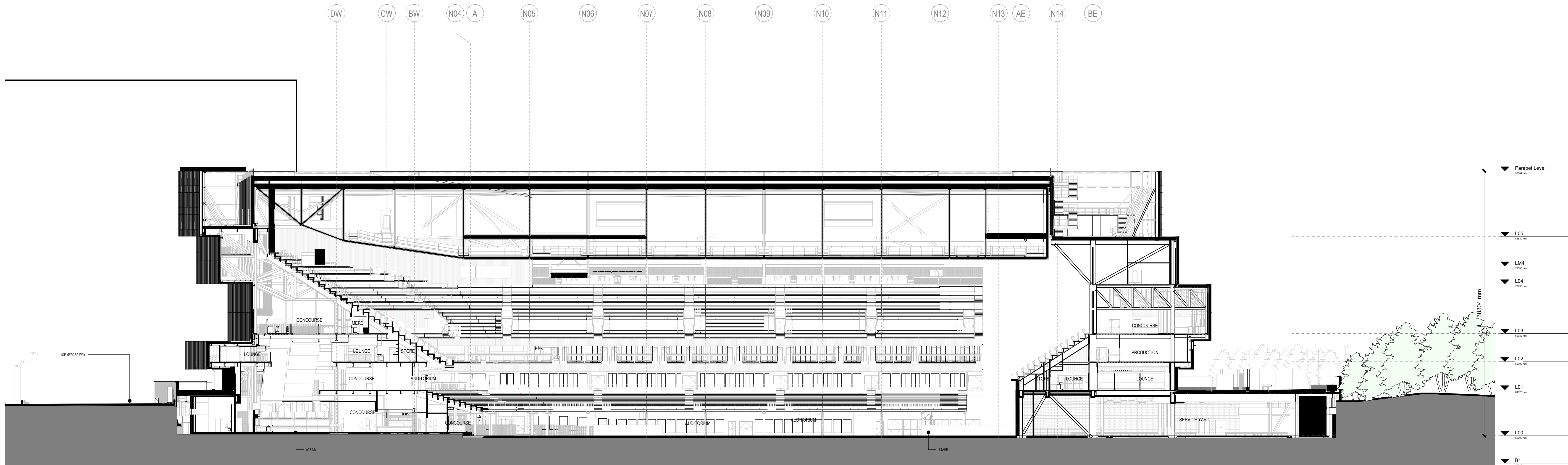
1 PLANNING SECTION - E/W - CENTRE 1:250
