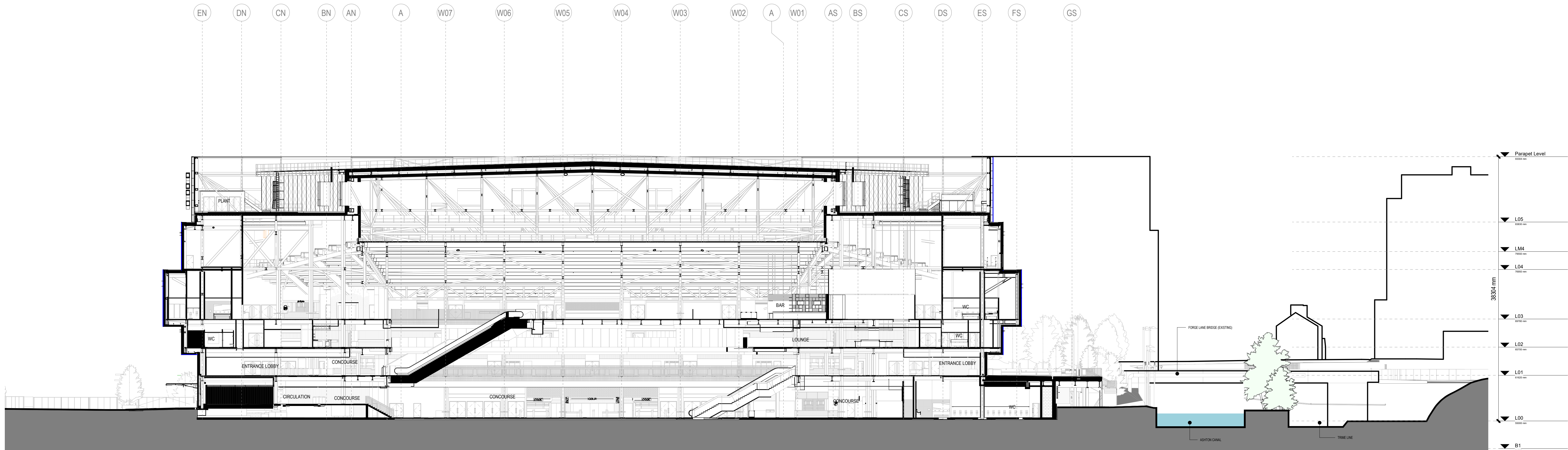
2 PLANNING SECTION - N/S - WEST ATRIUM 1:250
