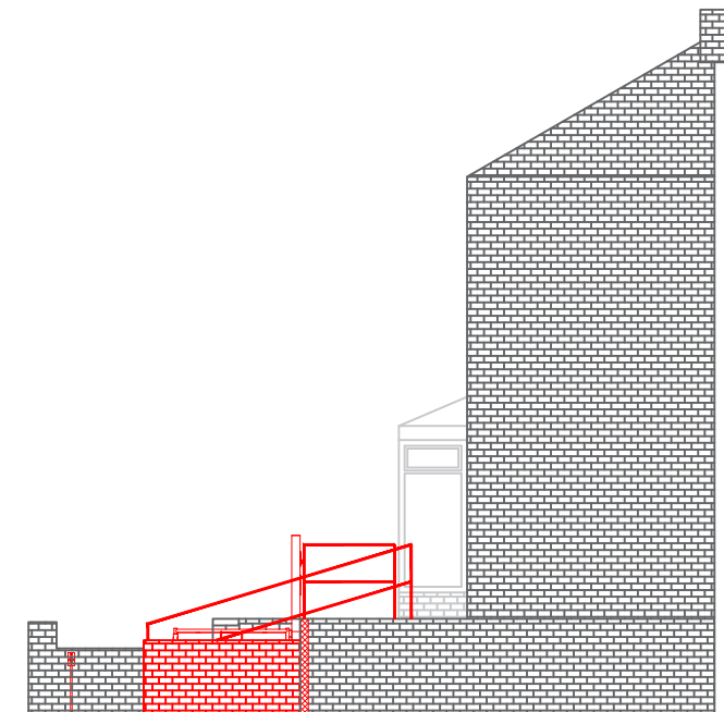
Proposed RHS Elevation
