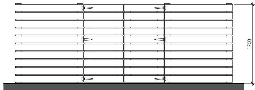
Bin Store - Front Elevation
