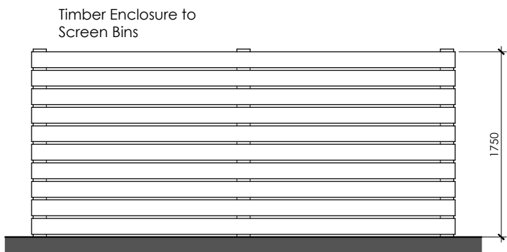
Bin Store - Side Elevations
