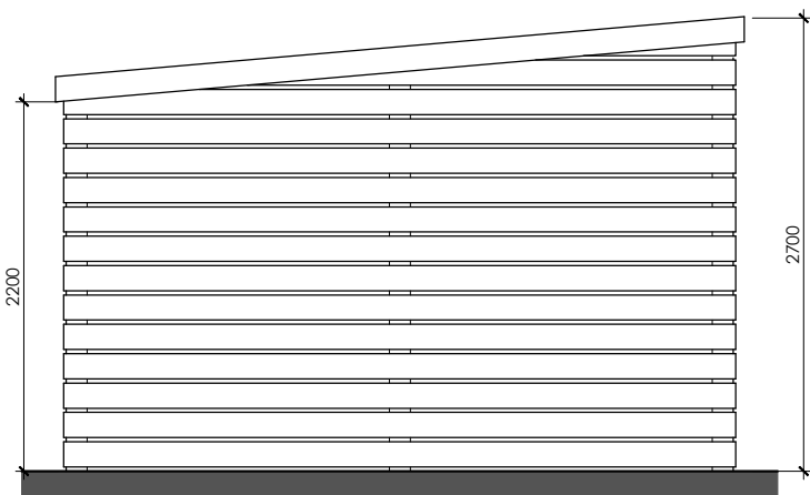
Cycle Store - Side Elevations
