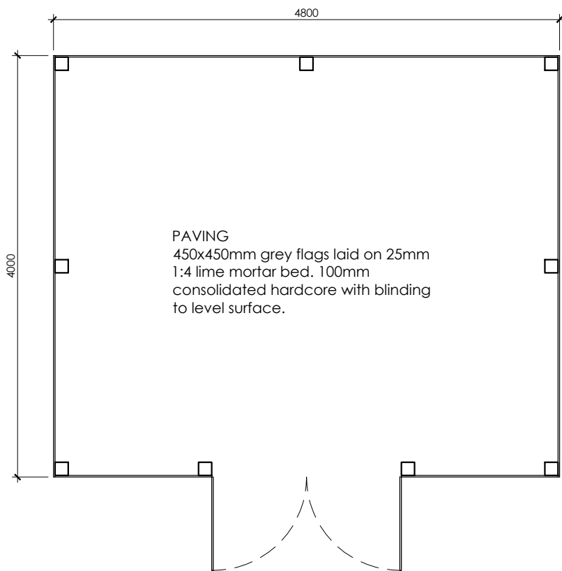
Bin Store - Plan
