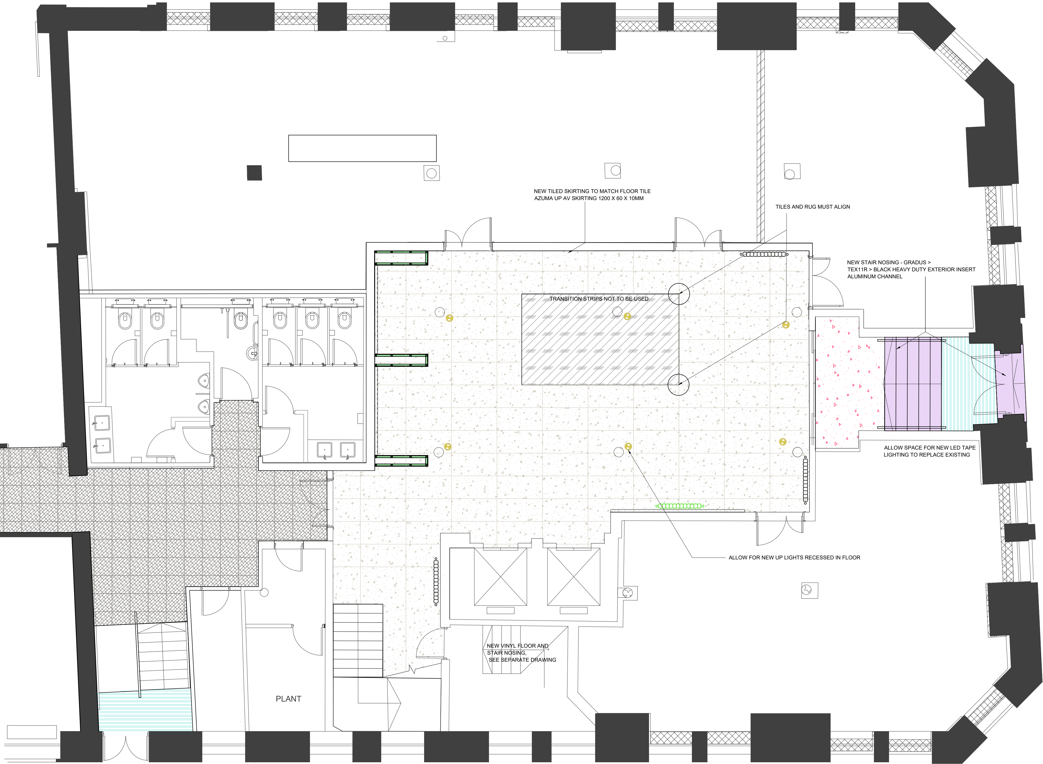
GROUND FLOOR
