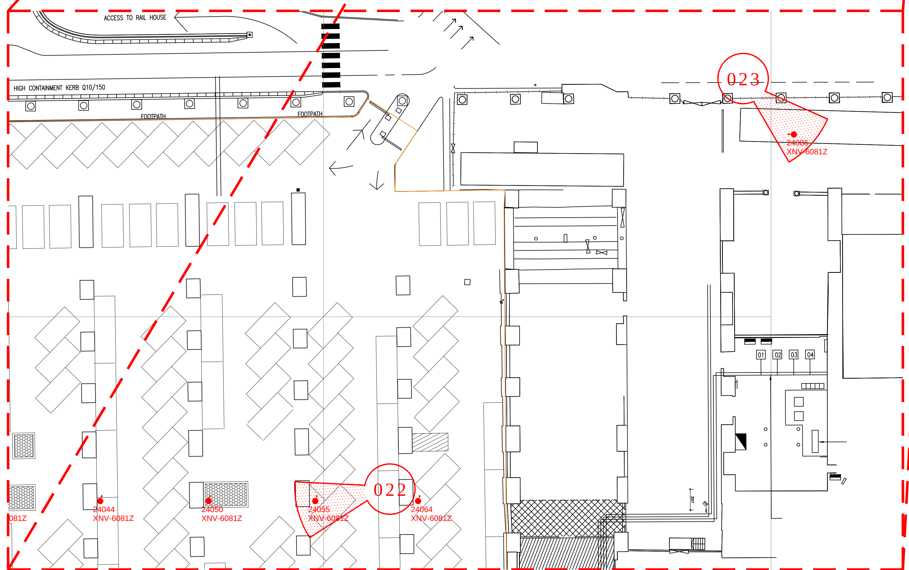
MANCHESTER PICCADILLY STATION PLAN UNDERCROFT - SCALE 1:250
