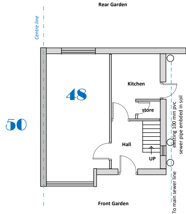
EXISTING DRAINAGE H. No. 48
