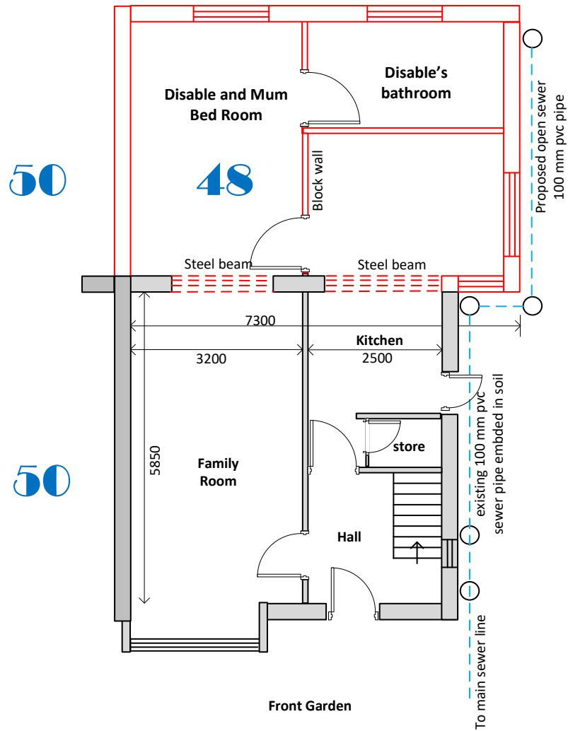
PROPOSED DRAINAGE House. No. 48
