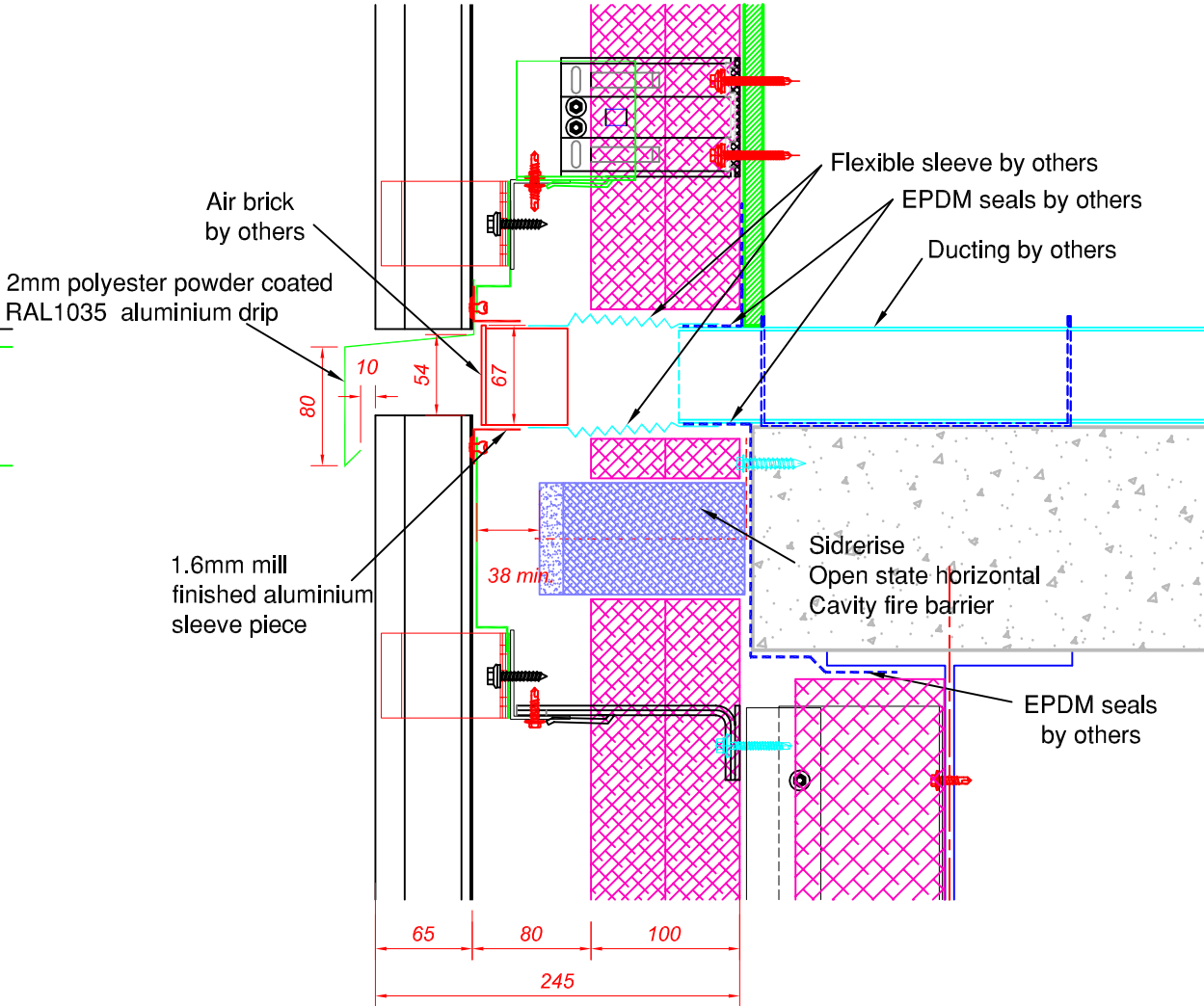
Section detail at each vent
