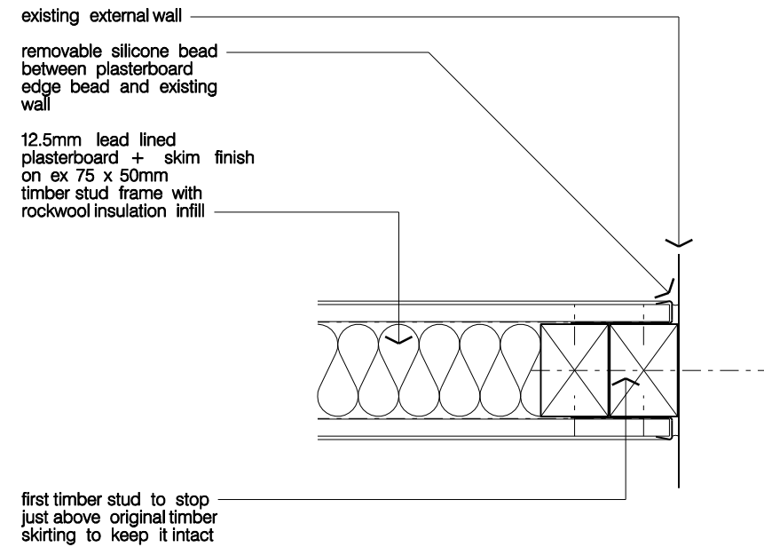
detail 3 new to old wall interface
