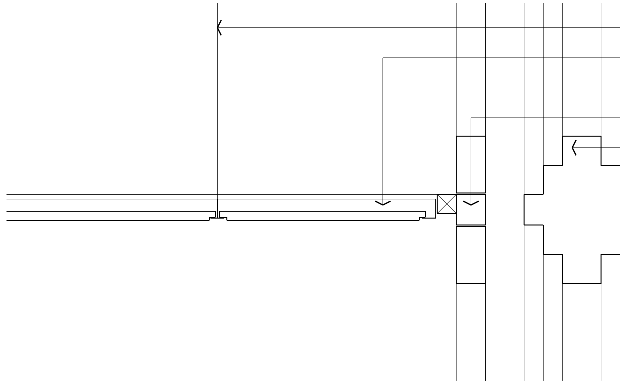
detail 1 section through proposed suspended ceiling
