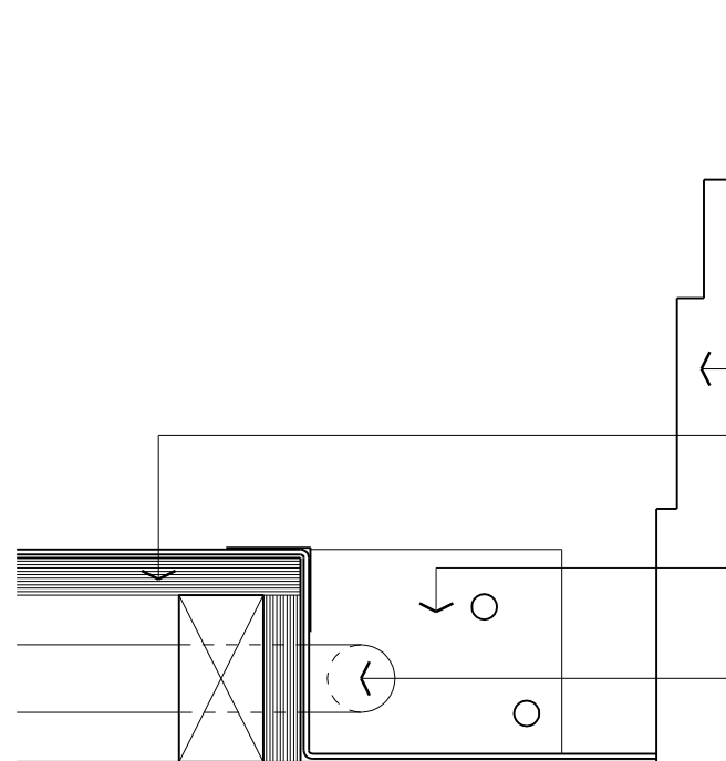
detail 2 section through new raised floor and service trench
