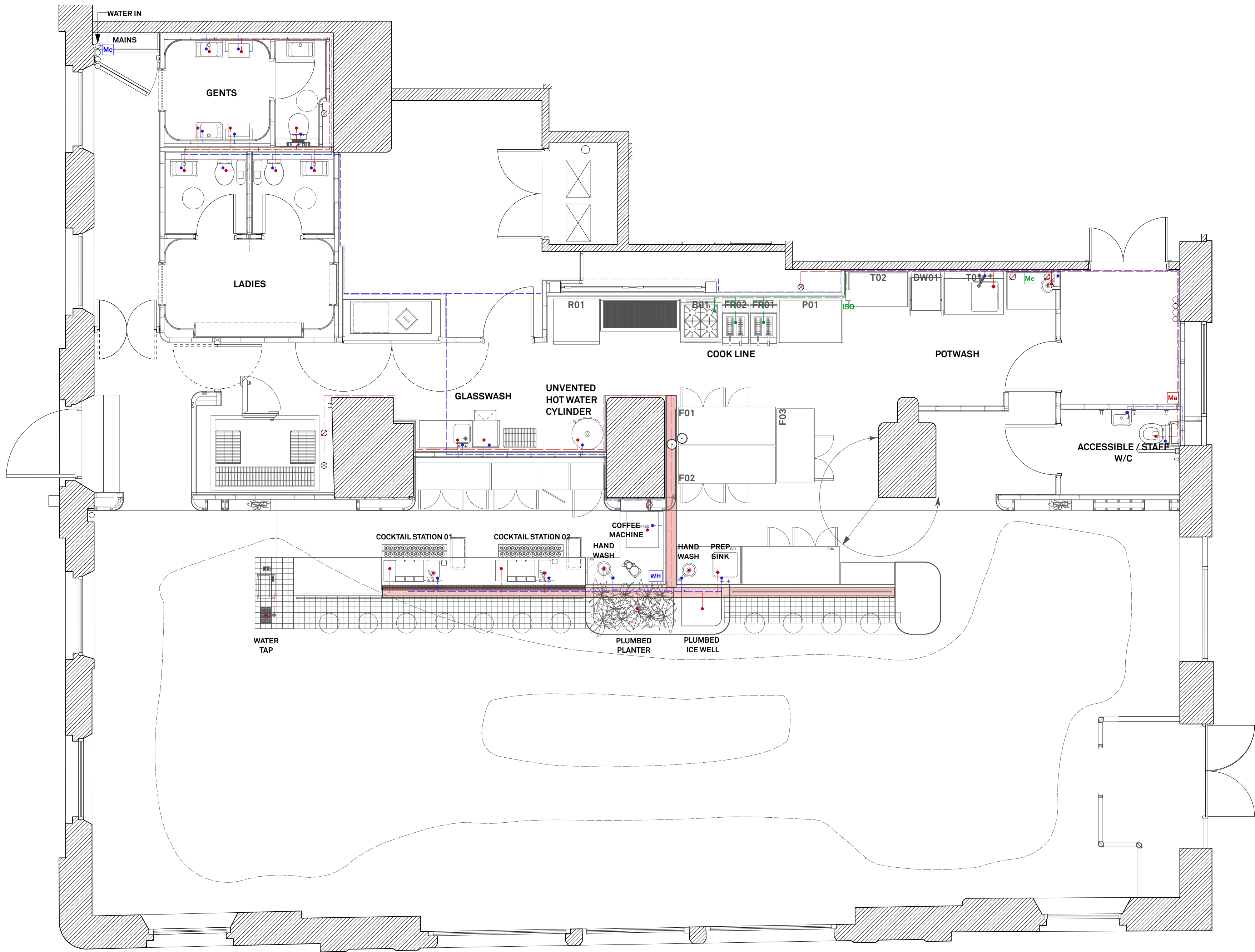
PROPOSED SERVICES PLAN Scale 1:50
