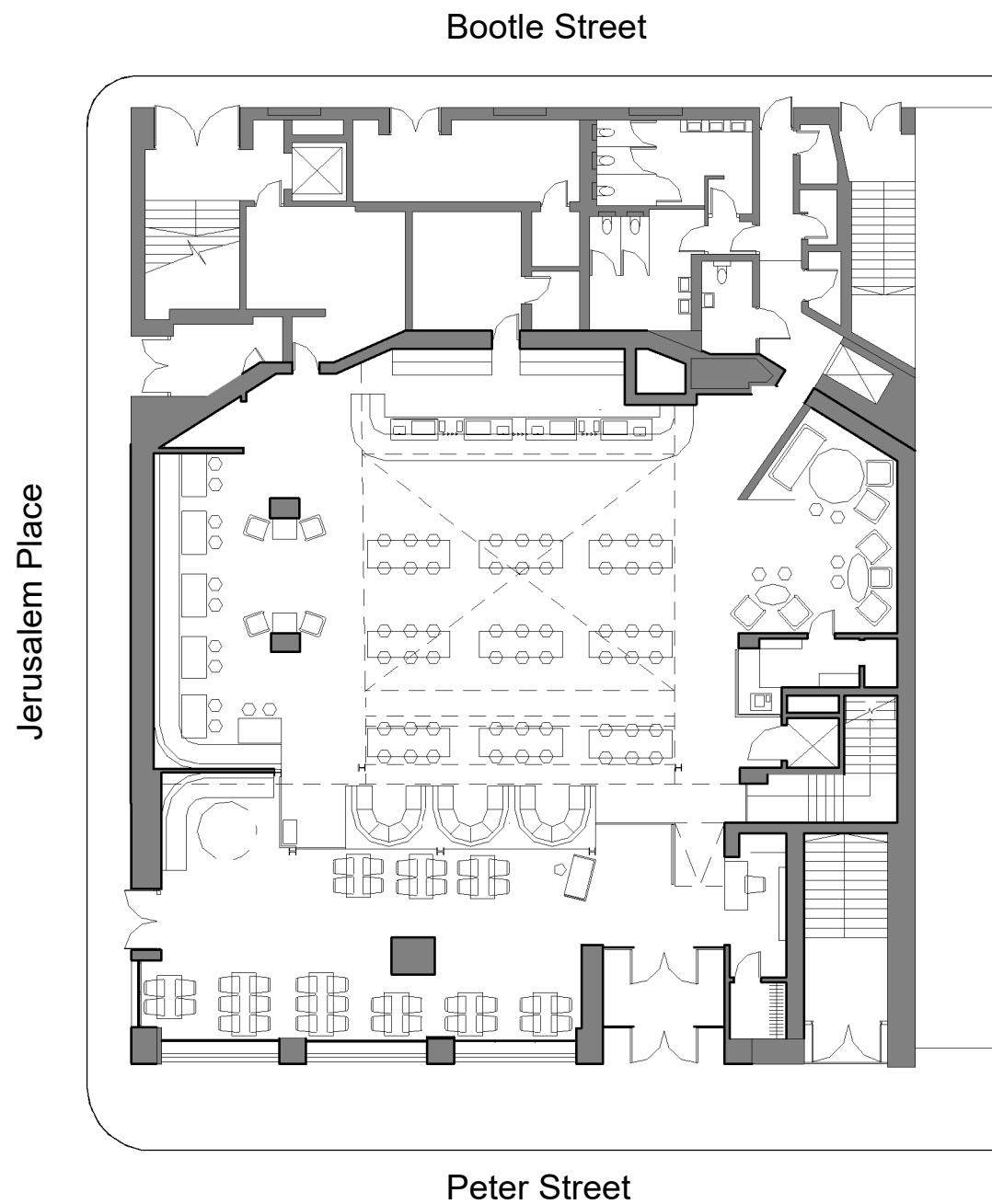
Existing Ground Floor Plan 1 : 200
