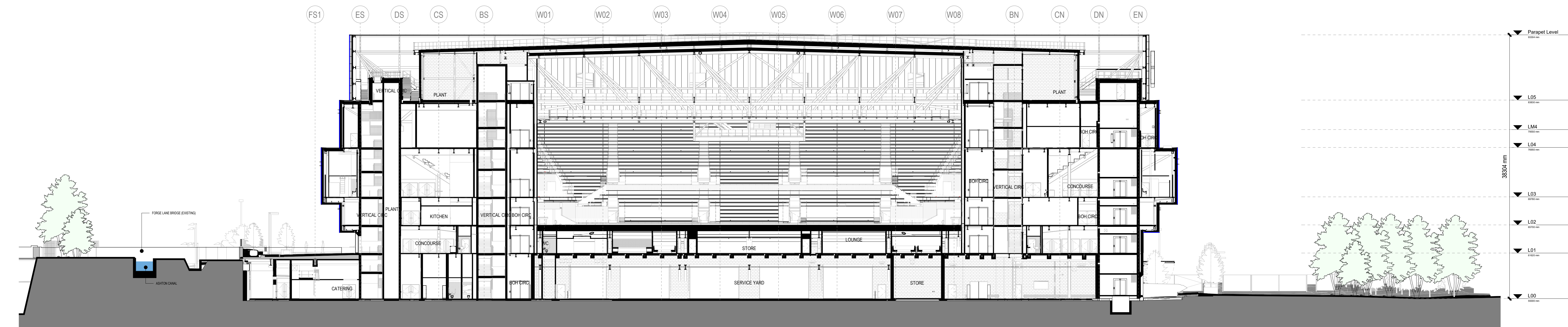
4 PLANNING SECTION - N/S - REAR STAGE TIER 1:250
