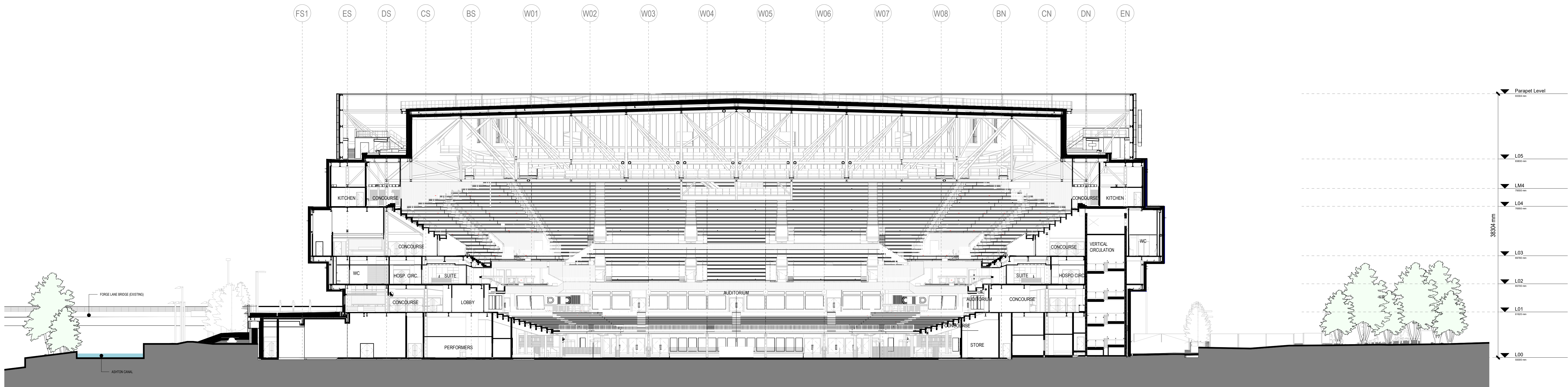
3 PLANNING SECTION - N/S - CENTRE 1:250
