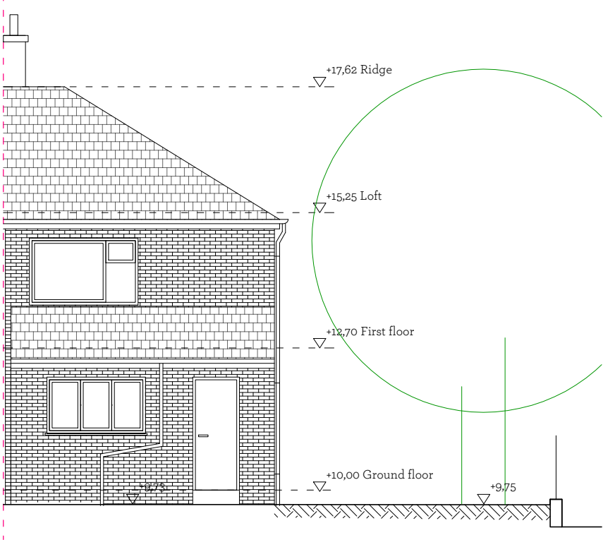
Garden Elevation
