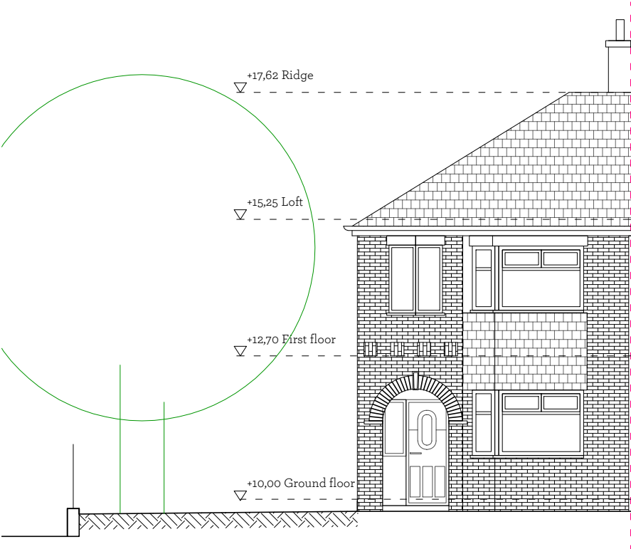
Front Elevation
