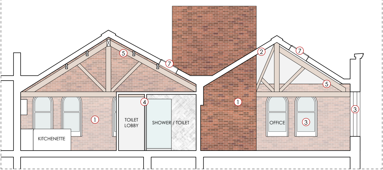
FOURWAYS HOUSE, FIFTH FLOOR PROPOSED SECTION CC'
