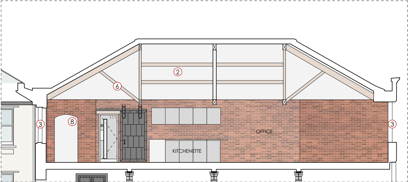
FOURWAYS HOUSE, FIFTH FLOOR PROPOSED SECTION DD'
