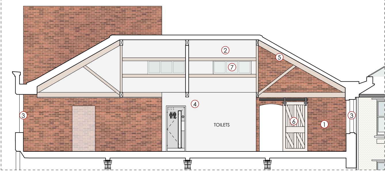
FOURWAYS HOUSE, FIFTH FLOOR PROPOSED SECTION EE'
