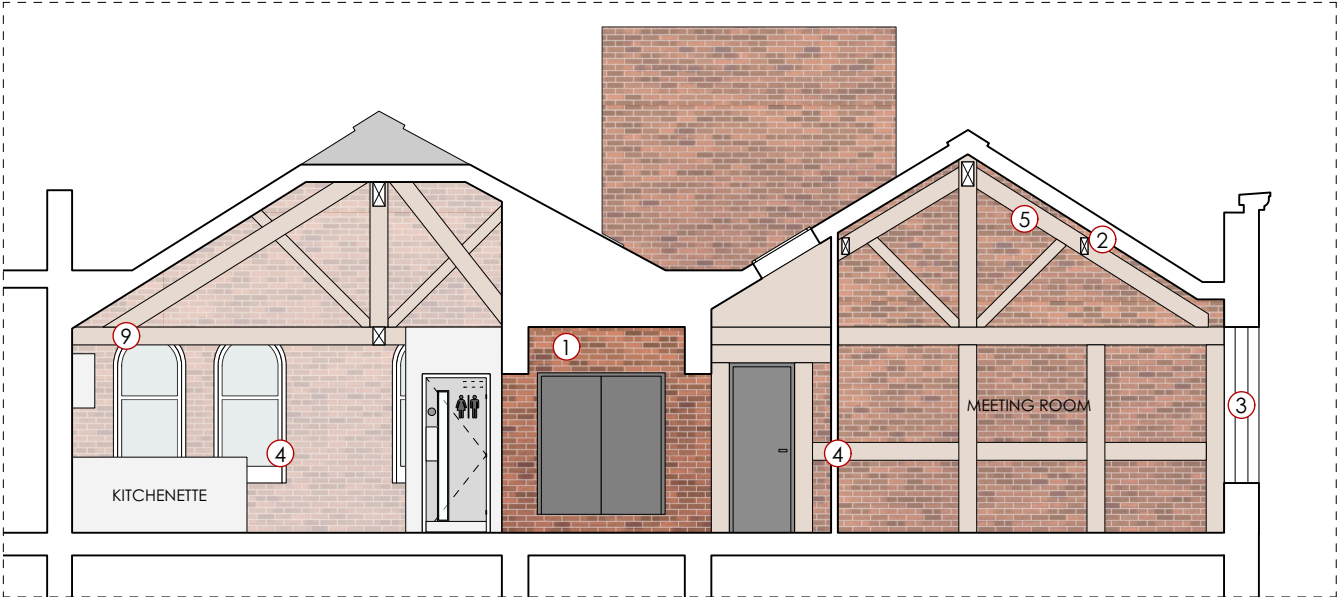
FOURWAYS HOUSE, FIFTH FLOOR PROPOSED SECTION BB'
