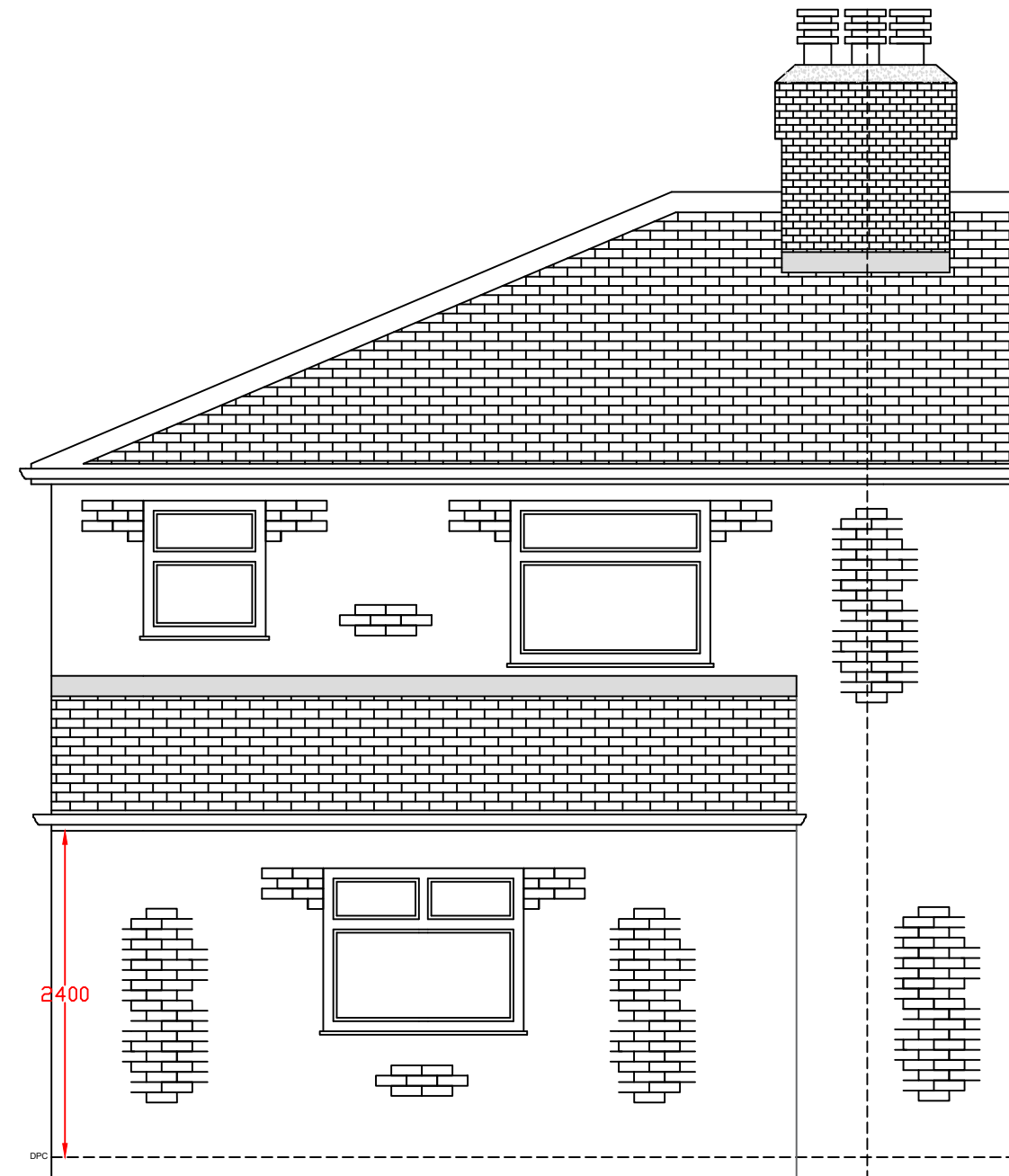
EXISTING FRONT ELEVATION (A) EXISTING REAR ELEVATION (B)
