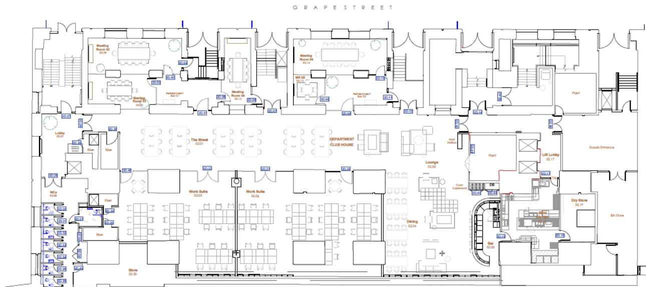
Figure 14: Proposed floorplan, Level 2 (2020). New bar, lounge and dining area to the east with work suites to the south and north sides, flanking the central 'street'. New WC facilities to be installed to the south west corner. Existing stairs and lift cores.
