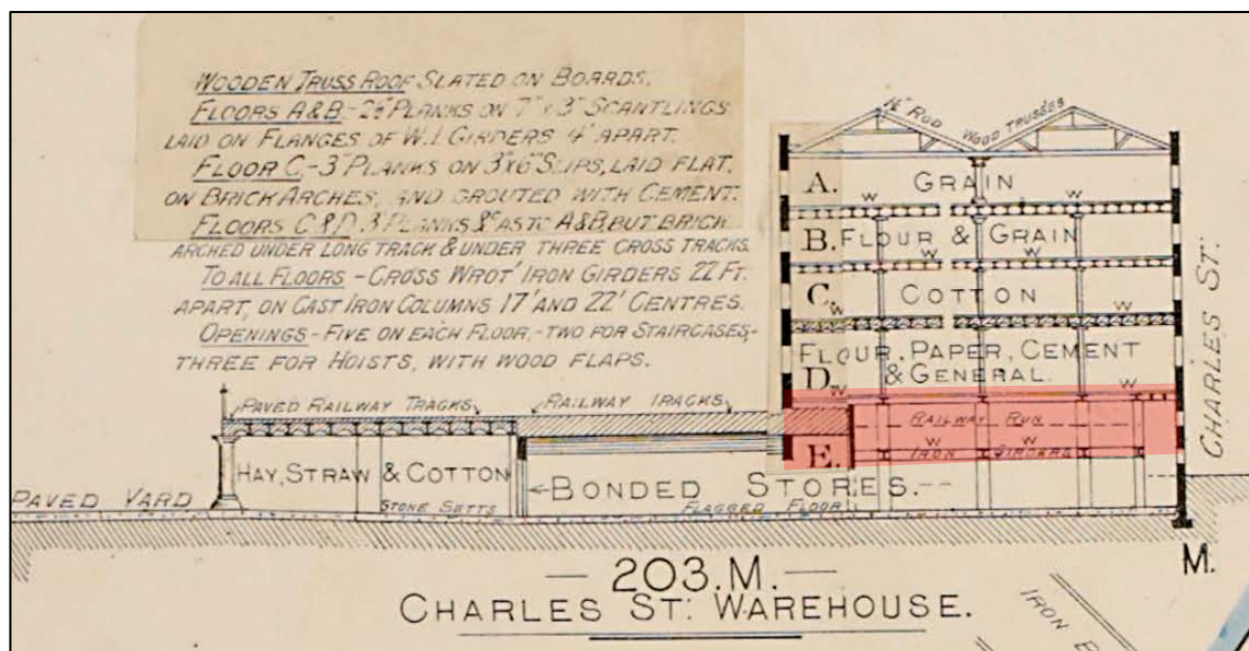
Figure 4: Cross section of the bonded warehouse from the Goad Map of 1888. The present day Level 2 is shaded red.
