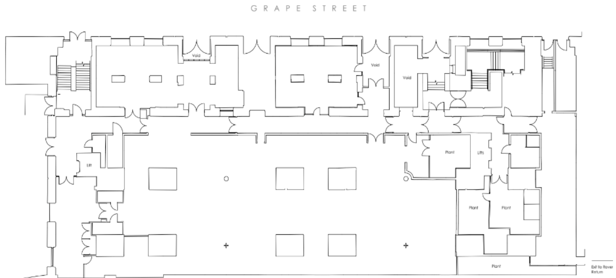
Figure 6a: The Bonded Warehouse c.2016. Level 2 floor plan. Note the original square brick piers which dominate the south side of the floorplate. The lightweight partitions and internal doors throughout are later additions.
