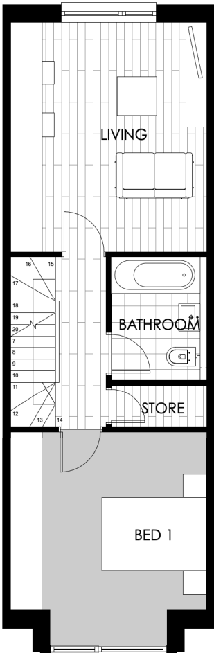
HOUSE TYPE 3A PROPOSED FIRST FLOOR PLAN
