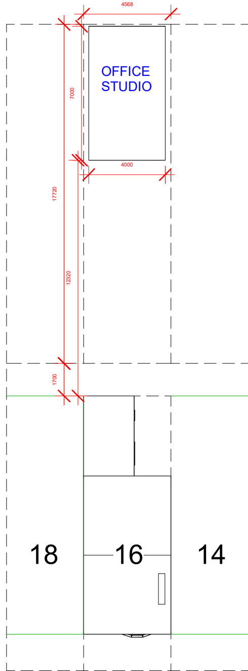
5 Proposed Site Plan 1 : 200
