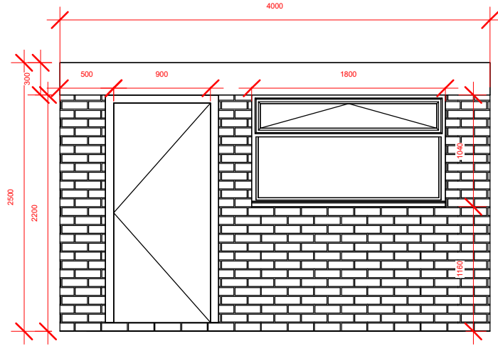
3 Front Elevation 1 : 50
