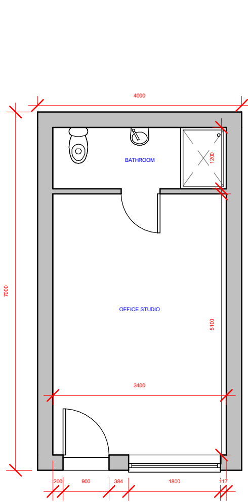
1 Proposed Setout 1 : 75
