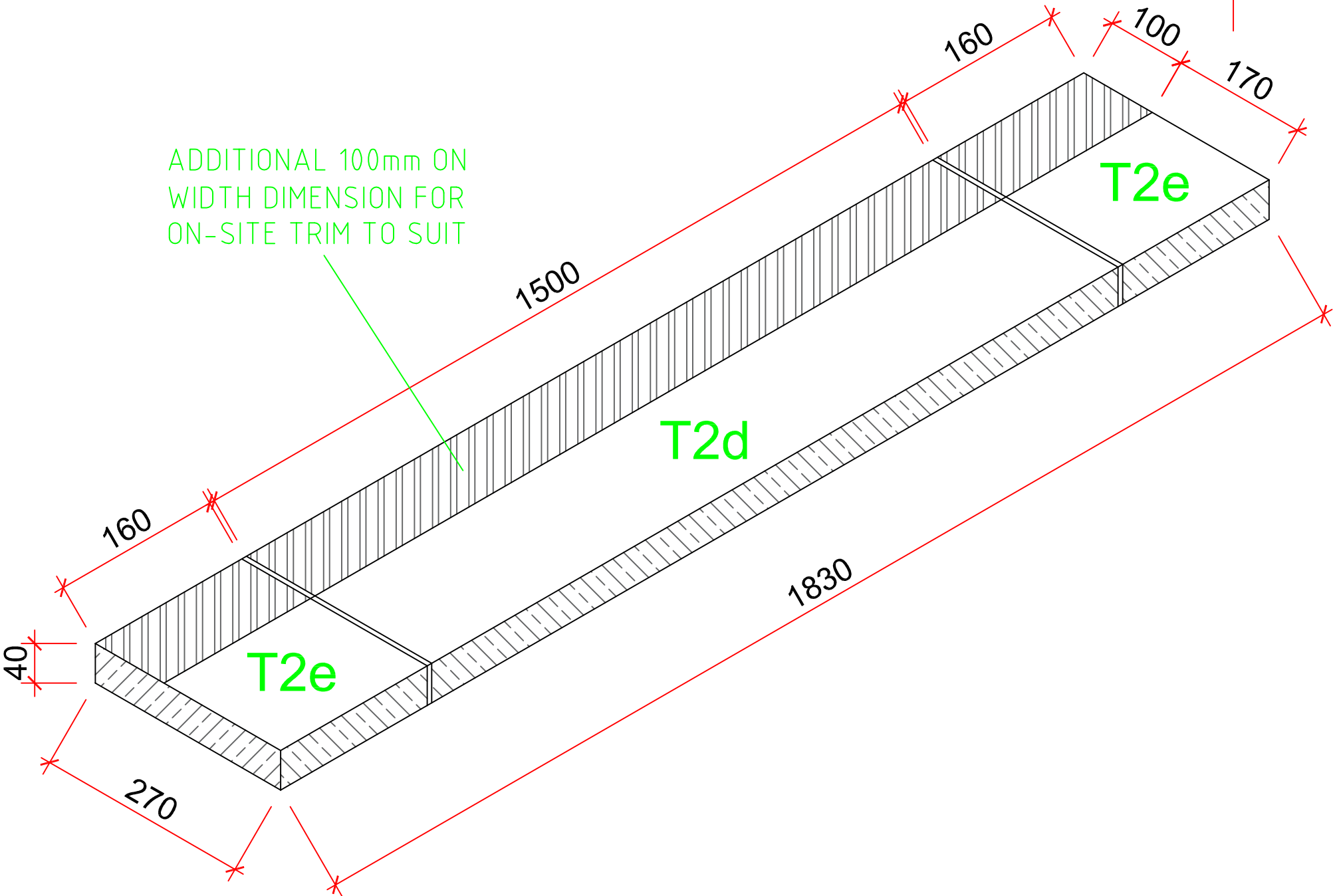
Step Flight No.1 Tread Plan Details (Step 4)
