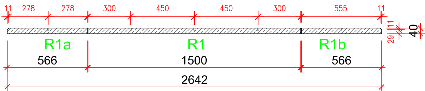
Step Flight No.1 Riser Plan Details (Step 1)
