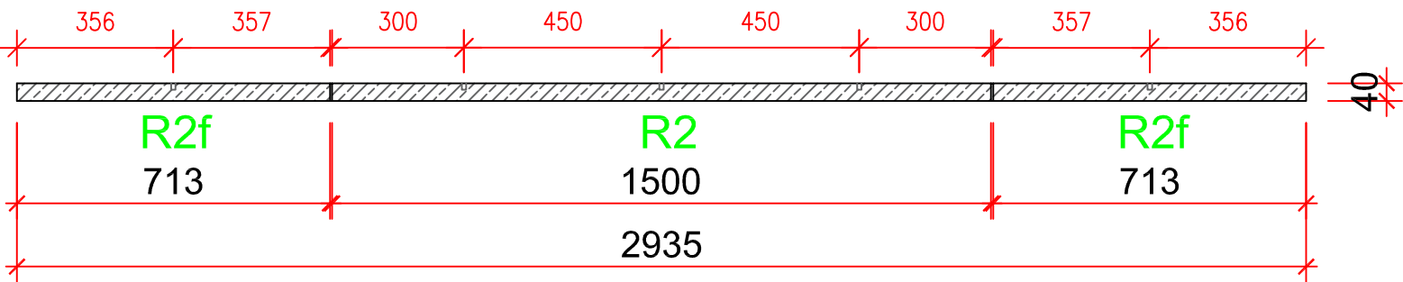
Step Flight No.2 Tread Plan Details (Step 1 to 7)
