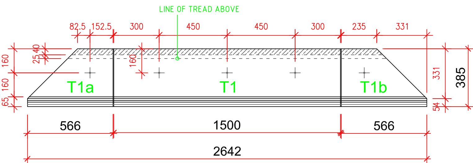
Step Flight No.1 Tread Plan Details (Step 1)
