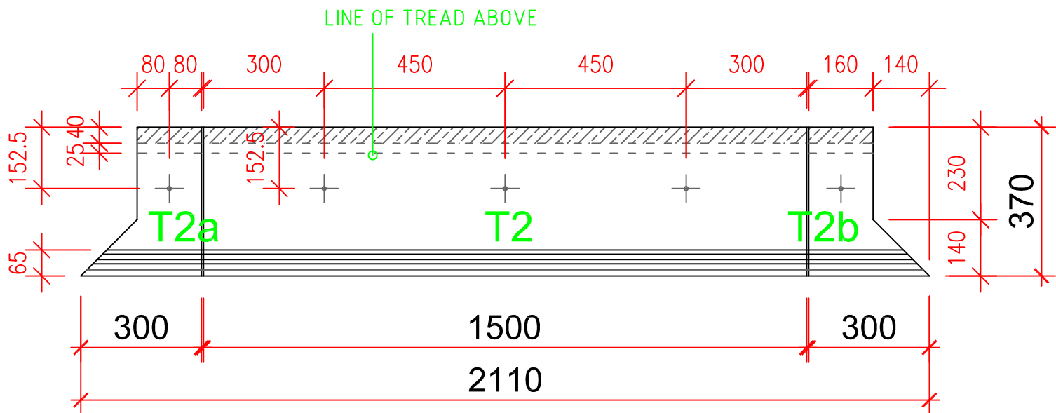
Step Flight No.1 Tread Plan Details (Step 2)
