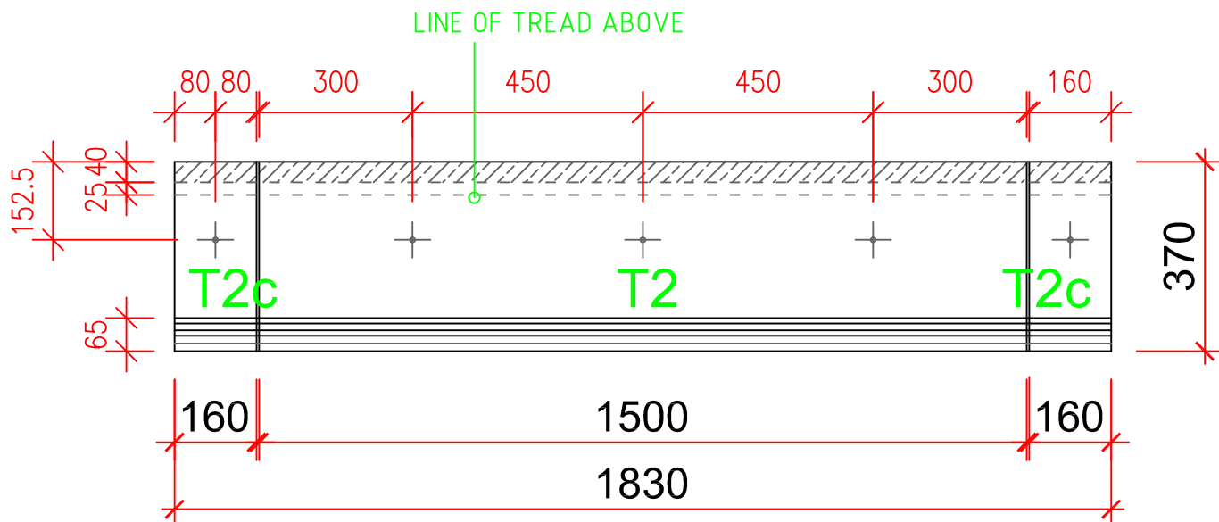
Step Flight No.1 Tread Plan Details (Step 3 & 4)
