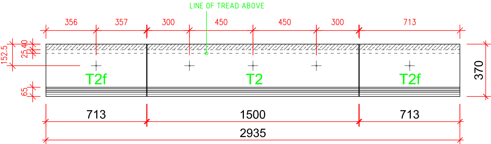
Step Flight No.2 Tread Plan Details (Step 1 to 7)
