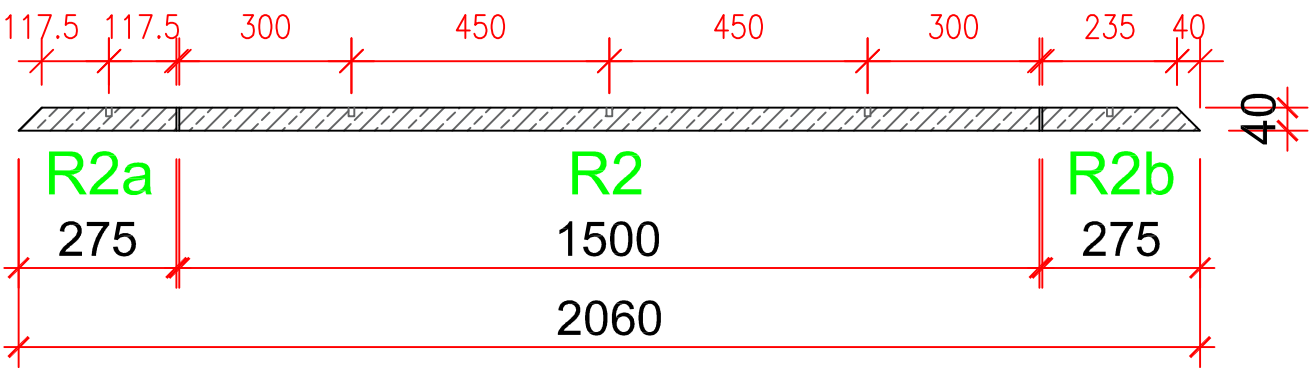
Step Flight No.1 Riser Plan Details (Step 2)
